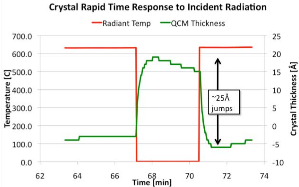
Figure 60. QCM rapid time response to incident radiation
