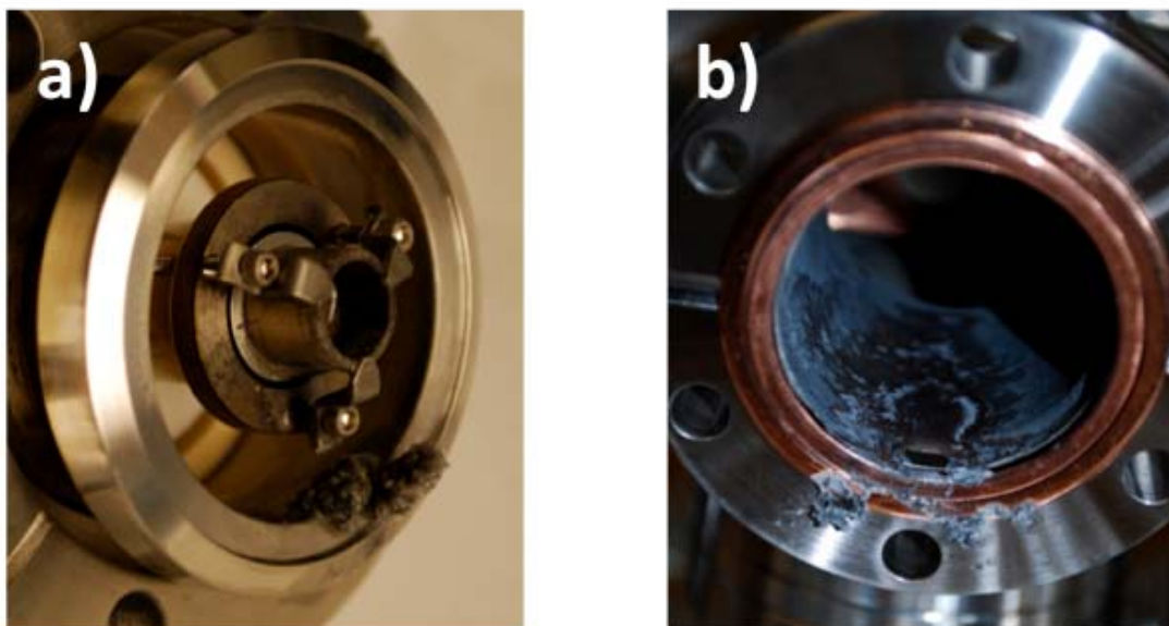
Figure 48. The heater and cartridge area after the 1 st Alvatec cartridge activation
