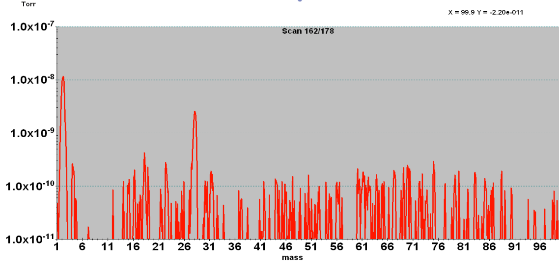
Figure 32. Representative RGA scan (at 6.80 V)
