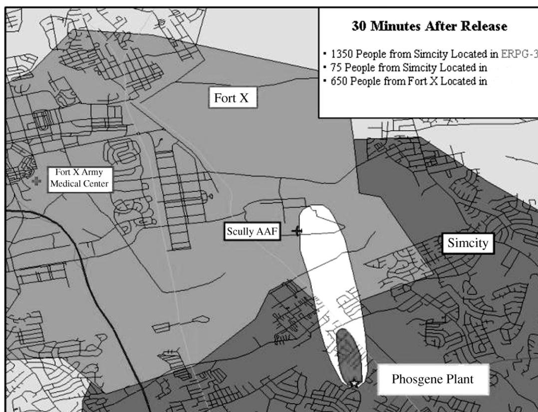
Fig. 2. Simulated downwind hazard areas for hypothetical release of phosgene gas.
