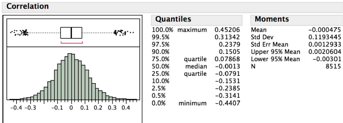
Figure 18. Distribution and Summary Statistics for the Factor Pairwise Correlations for Design Points yielding MOE 3 results
