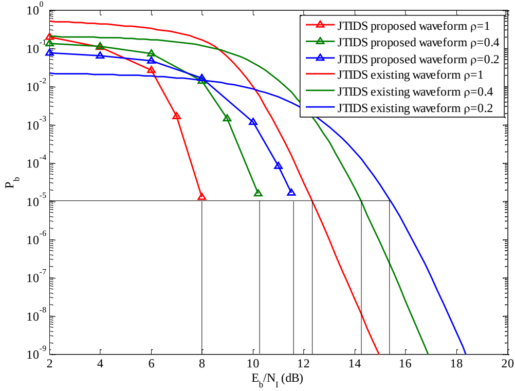
Figure 62. Performances of the proposed and existing Link-16/JTIDS waveforms for noncoherent demodulation in AWGN and PNI.
