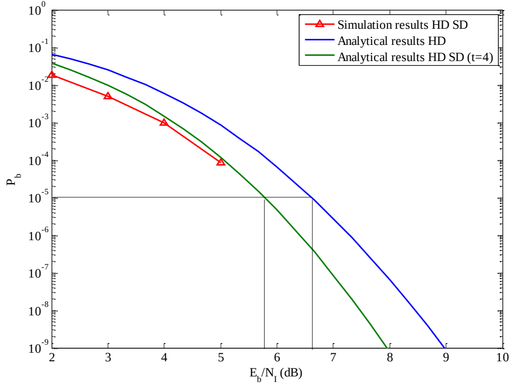
Figure 27. Probability of bit error for single-symbol 16-FSK with (15, 9) RS encoding in both AWGN and PNI for \rho = 1 and E_b/N_0 = 13\text{dB} .
