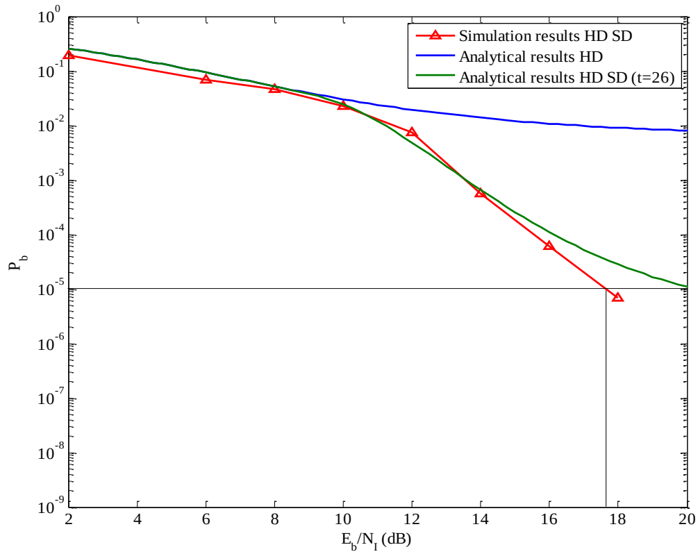
Figure 53. Probability of bit error for double-symbol 16-FSK with (255, 223) RS encoding in both AWGN and PNI for \rho = 1 and E_b/N_0 = 5.3\text{ dB} .
