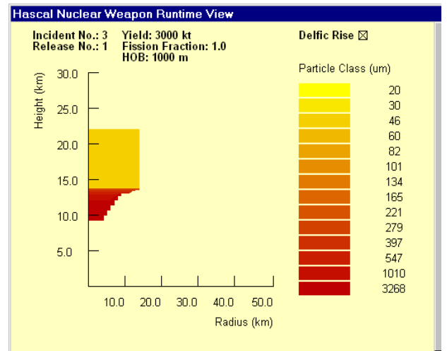
Figure 3 Particle size distribution of the initial cloud as determined by NewFall.
