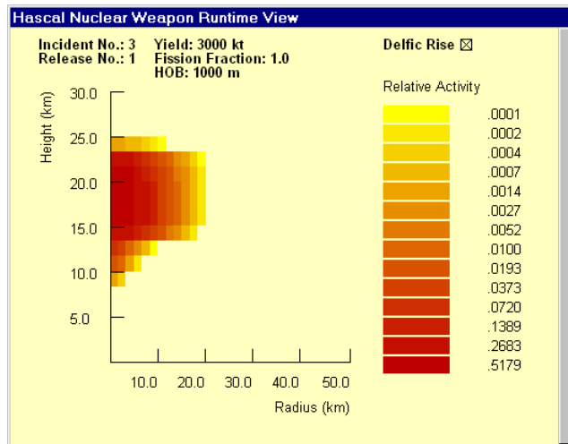
Figure 2 Relative radioactivity as a function of height of the initial cloud as determined by NewFall.
