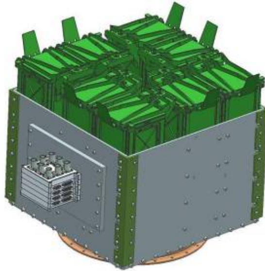
Figure 4 NPSCuL-Lite integrated with P-PODs (From [22])
