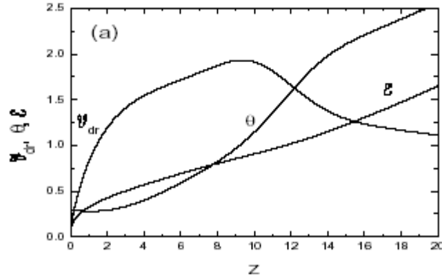
Fig. 13. Characteristic dimensionless drift velocity, electron temperature and local electric field v_{dr}(z) , \theta(z) , and \varepsilon(z) for spatially dependent transport in nitride short diodes at a given current density 1.1 \text{ kA/cm}^2 . The parameters v_{dr}(z) and \varepsilon(z) are scaled to V_O and F_O given in Table 2. The electron temperature \theta(z) is scaled to the optical phonon energy ( \approx 92 \text{ meV} \approx 1060 \text{ K} for GaN). The coordinate z is measured in units l_O .
