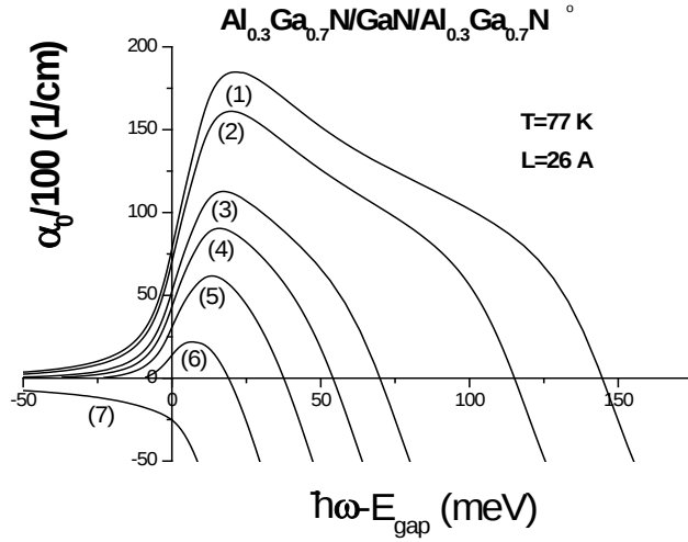
Fig. 11. Specific amplification for a single quantum well of thickness 26 Å at the nitrogen temperature. The curves 1 through 7 corresponds to plasma concentrations 10^{13} \text{ cm}^{-2} , 8 \cdot 10^{12} \text{ cm}^{-2} , 5 \cdot 10^{12} \text{ cm}^{-2} , 4 \cdot 10^{12} \text{ cm}^{-2} , 3 \cdot 10^{12} \text{ cm}^{-2} , 2 \cdot 10^{12} \text{ cm}^{-2} and 10^{12} \text{ cm}^{-2} .
