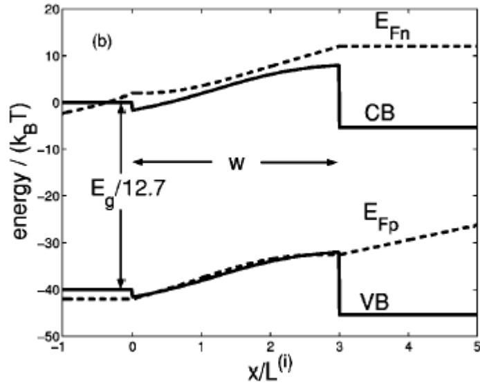
Fig. 8. The energy band diagram of the structure calculated in Fig. 7. CB and VB indicate the lowest populated energy levels in conduction and valence bands, respectively. Quasi-Fermi levels for the electrons and holes are shown.
