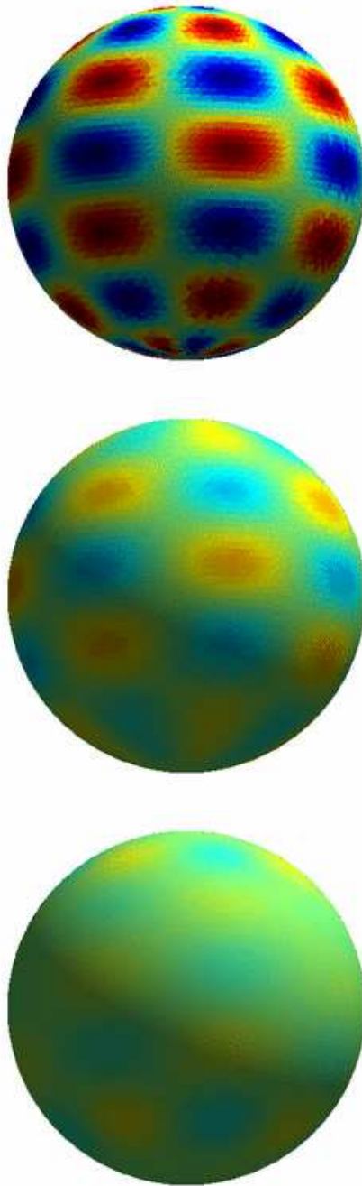
Figure 3: Linear fourth order diffusion on the sphere after 0, 4, and 18 time steps. Red denotes u = 1 and blue denotes u = -1 .
