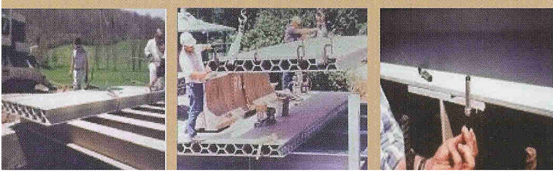
Figure 4. West Virginia University FRP composite bridge deck projects. (A) FRP deck panel field installation using adhesive bonding. (B) Preparing to apply second FRP deck panel section. (C) Panels are connected to stringers using mechanical fasteners and adhesive bonding.
