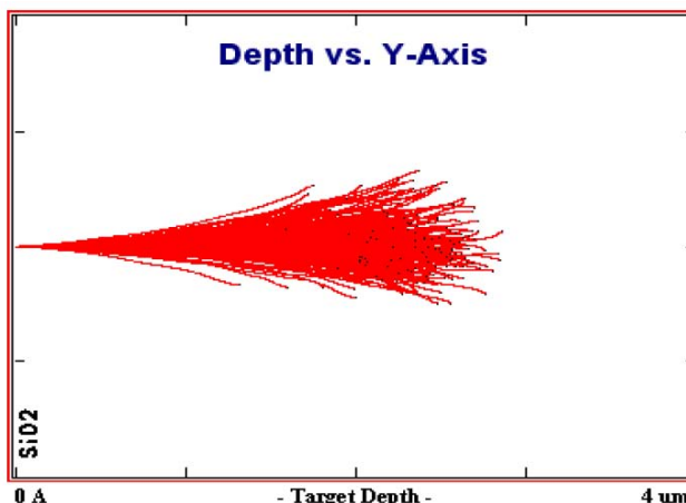
Figure 1 TRIM calculation of penetration depth of 10 MeV Pt ions implanted into silica matrix.
