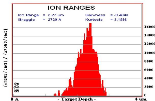
Figure 2 Ion stopping range to ensure the employed ions having high enough energy capable of penetrating through a 1-micron sized silica sphere.
