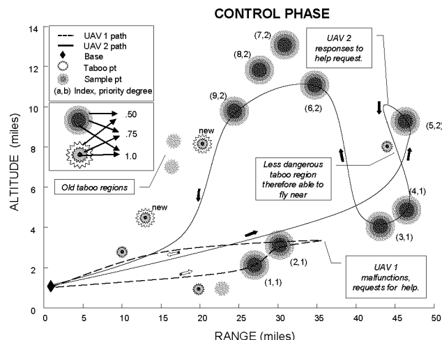
Figure 3: During flight, updates about environmental changes cause the real-time control algorithms on the two UAVs to change their trajectories.
