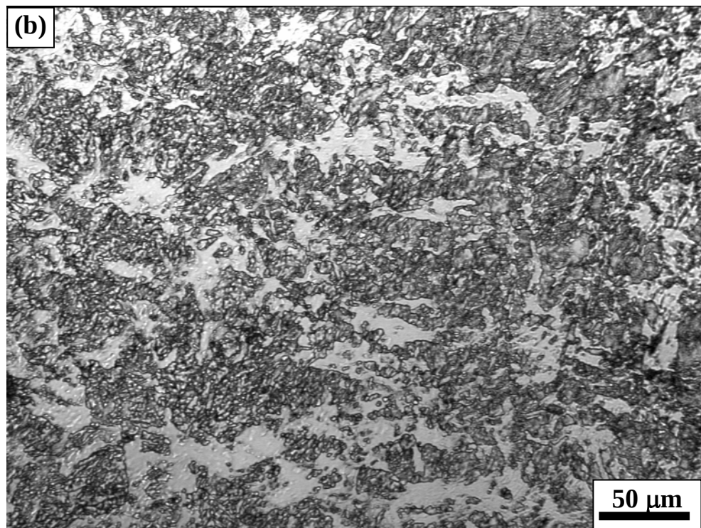
Fig. 7. Metallographic pattern of W after ECAP by regime: 2 cycles at 1200 ^{\circ}\text{C} +2 cycles at 1100 ^{\circ}\text{C} and 2 cycles at 1000 ^{\circ}\text{C} : a- longitudinal, b- cross sections
