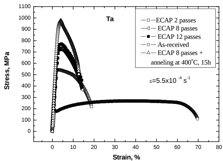
Fig. 16. Engineering tensile curves of Ta before and after ECAP with a different number of cycles
