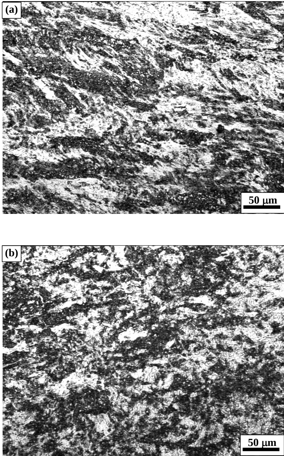
Fig. 10. Metallographic pattern of W after 8 ECAP cycles at 1150 °C: a- longitudinal section, b- cross section
