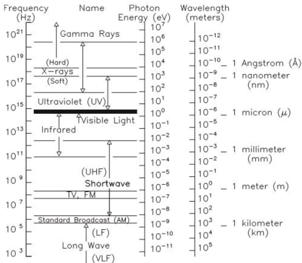
Figure 3. Electromagnetic Spectrum (From Olsen 34)
