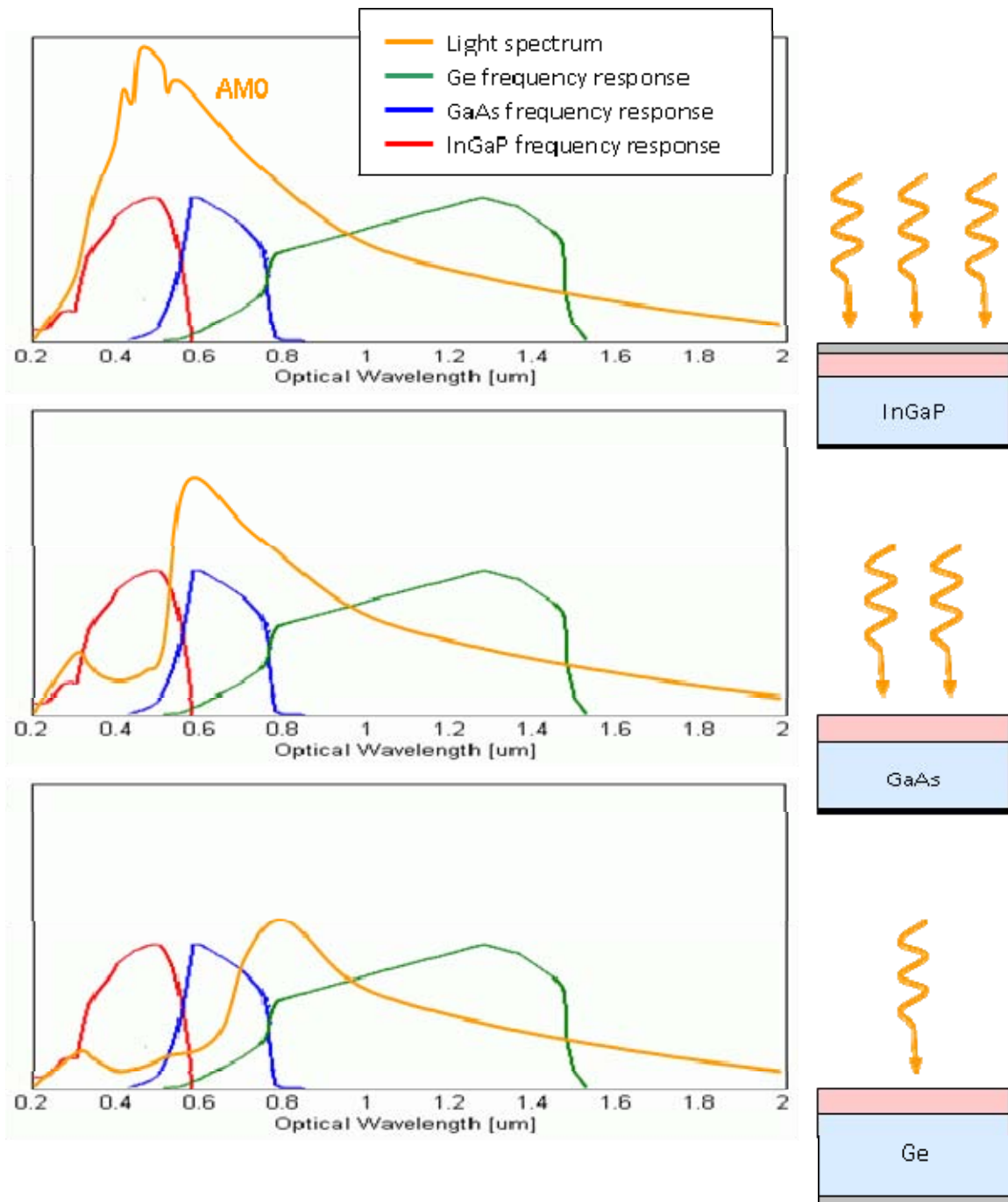
Figure 28. Available Solar Spectrum Peak Shift (From Michalopoulos 121)
