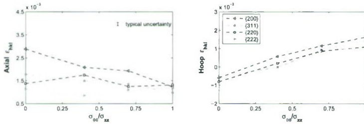
Figure 11: Biaxial loading experiments: measured axial and hoop lattice strains grouped by (hkl) taken from Figure 10 at an axial stress of 370MPa for various levels of stress biaxiality.
