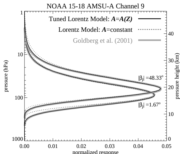
Fig. 3. Channel 9 1-D vertical temperature weighting functions W_j(Z) for the smallest off-nadir angle of \beta_j=\pm 1.67^\circ and largest off-nadir angle of \beta_j=\pm 48.33^\circ , derived from our simple Lorentz model (constant A ; dotted curve) and tuned Lorentz model (height-varying A , solid curve). Gray curves show results of Goldberg et al. (2001) using a complete radiative transfer model.
