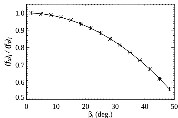
Fig. 5. Ratio of along-track to cross-track footprint diameters (f_X)_j / (f_Y)_j versus scan angle \beta_j based on Eqs. (9) and (10) for NOAA satellite orbit parameters and a nominal Channel 9 measurement altitude of Z_C=18 \text{ km} .
