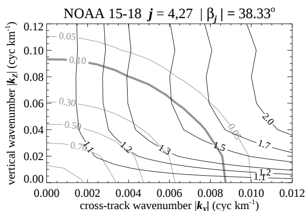
Fig. 15. Black contours show the spectral variance visibility ratio \hat{R}_{j,j_*}^2(k_Y, k_Z) as a function of cross-track and vertical wavenumber for the NOAA AMSU-A j=4 , j_*=27 conjugate beam pairing. Gray lines overlay absolute visibility contours of \hat{W}_j(k_Y, k_Z) for the j=4 beam.
