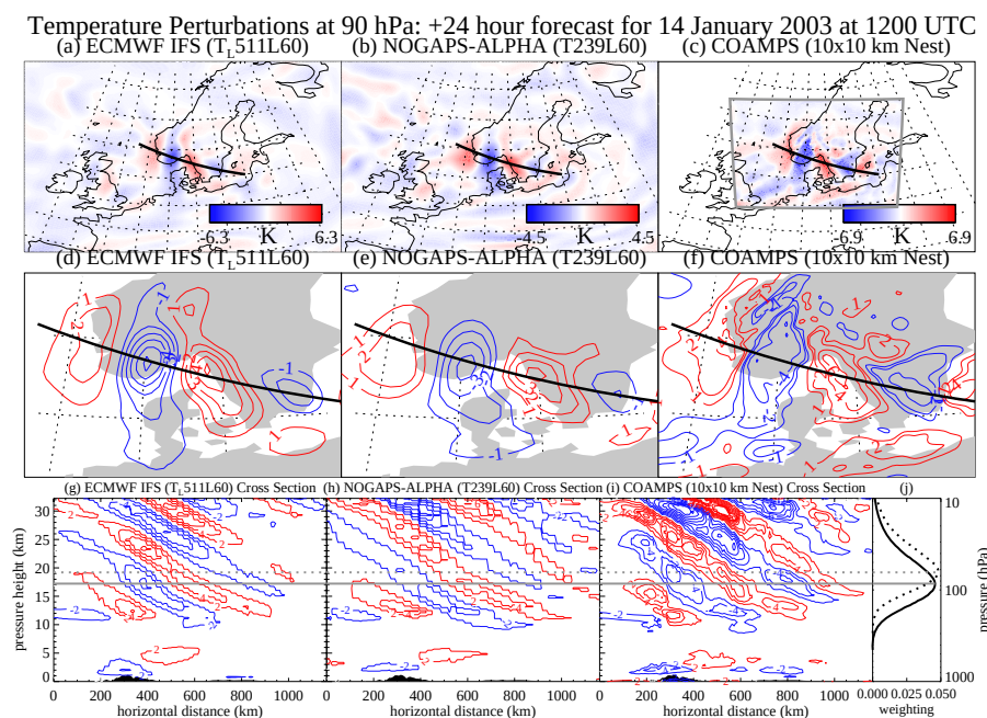
Fig. 8. Top row plots temperature perturbations T'(\lambda, \phi, p) at p=90 hPa extracted from +24 h forecasts from ECMWF IFS (left column), NOGAPS-ALPHA (middle column) and COAMPS (right column) runs, using a similar map range to AMSU-A brightness temperature perturbations in Fig. 6. See color bar in the lower-right corner of each panel for temperature range. Middle row plots same fields, but now focused over southern Scandinavia. Contour interval is 1 K. Bottom row of plots shows altitude contours of T'(\lambda, \phi, p) along the horizontal cross section plotted as black curve in the panels above. Negative (cold) temperature anomalies are blue, positive (warm) temperature anomalies are red, and the contour interval is 2 K (zero contour is omitted). Cross sections of topographic surface elevations are shaded in gray. Panel (j) replots AMSU-A Channel 9 1-D vertical weighting functions from Fig. 1b.
