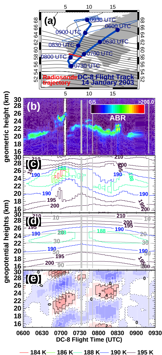
Fig. 11. (a) Blue curves show DC-8 flight of 14 January 2003, with period from 06:00–09:30 UTC highlighted with thicker curve and 30 min markers. Red curve shows horizontal radiosonde trajectory from Fig. 9. Contours show 12:00 UTC 925 hPa NAVDAS analyzed geopotential heights. (b) S_{1064} from GSFC/LaRC aerosol lidar from 06:00–09:30 UTC, derived as 8 point averages of the raw data (4 points in time, 2 points in height). Gray strips omit data where DC-8 turned in (a) to roll angles >5^\circ which tilted the lidar beam off zenith. Color bar scale is logarithmic. (c) Temperatures T along DC-8 flight track from NOGAPS-ALPHA +19 h forecast, valid at 07:00 UTC, plotted versus model geopotential height. Contour color scale is shown beneath panel (e). (d) as for (c) but plotting mean temperatures \bar{T} . Gray contours show pressure surfaces in hPa. (e) as for (c) but plotting temperature perturbations T' , the difference field between (c) and (d). Contour interval is 2 K, positive values are red and negative values are blue.
