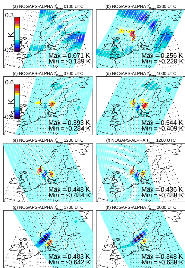
Fig. 16. Similar presentation to Fig. 6, but showing brightness temperature perturbations T'_{B\text{NWP}}(\hat{\lambda}_j, \hat{\phi}_j) derived via Eqs. (2) and (6) from the hourly NOGAPS-ALPHA temperature hindcast field closest in time to the satellite overpass in question. Values are in Kelvin (see color bars): for panels (a) and (b) the range is \pm 0.3 K, whereas for panels (c–h) the color bar range is \pm 0.6 K. Maximum and minimum values for each map are shown in the lower-right portion of each panel.
