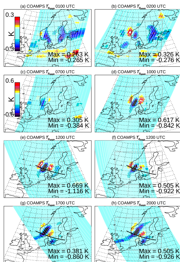
Fig. 17. Same presentation as Fig. 16, but showing brightness temperature perturbations T'_{B\text{NWP}}(\hat{\lambda}_j, \hat{\phi}_j) derived from hourly COAMPS temperature fields. Gray curve shows borders of the COAMPS domain. Black curves in panels (e–h) reproduce the cross section from Figs. 7a and 8 along which brightness temperatures are profiled in Fig. 18.
