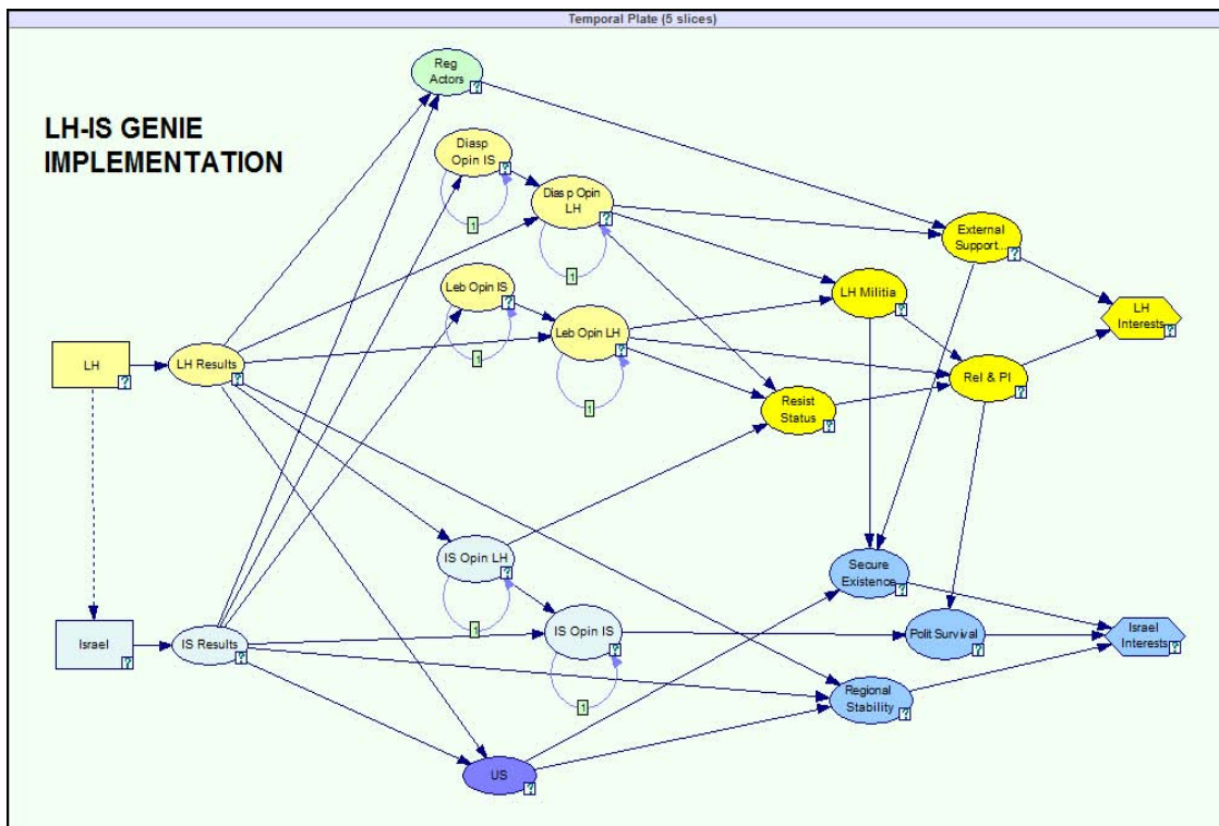
Figure 9. The LH-IS model implemented in the Genie v2.0 user interface.
