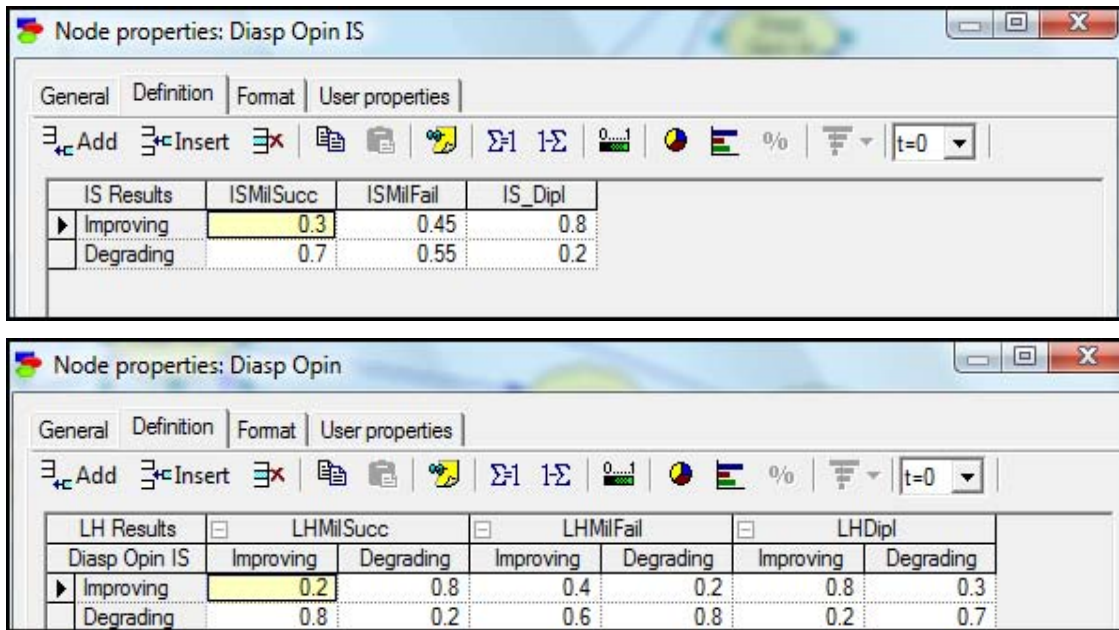
Figure 10. Example of probability table in Genie v2.0, using Diaspora as an example.
