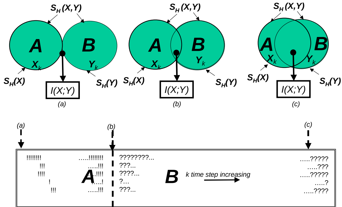
Figure III-10 Interacting Systems A and B
