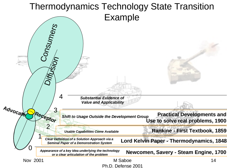
Figure II-8 Thermodynamics Technology Transition State Example
