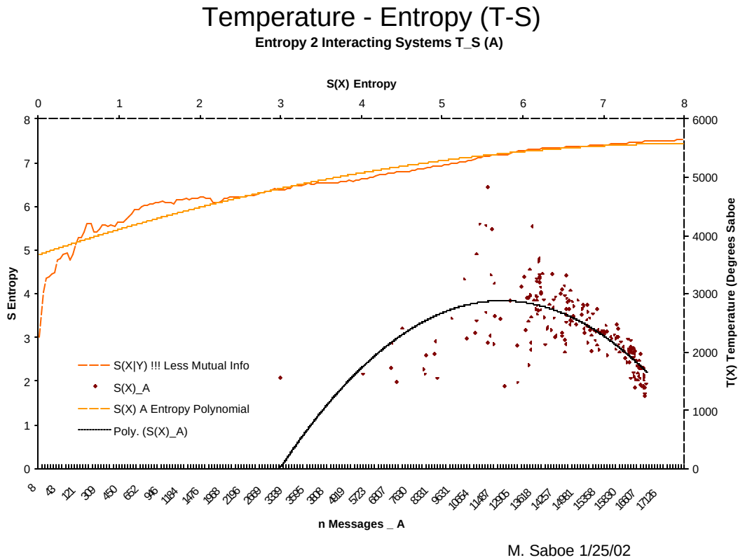
Figure III-16 Entropy -- Messages, and Temperature – Entropy
