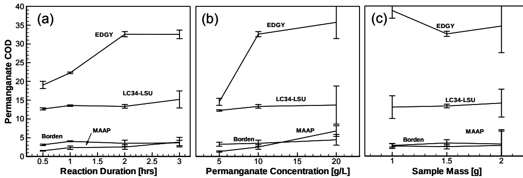
Figure 20: Sensitivity of the permanganate COD test results due to changes in (a) reaction duration, (b) initial permanganate concentration, and (c) sample mass of aquifer material. All test values are expressed in terms of g of \text{KMnO}_4 per kg of dry aquifer material. The error bars represent \pm one standard deviation.
