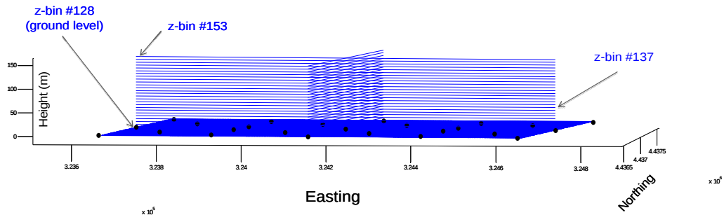
Figure 22. AIRIS z-bins.
