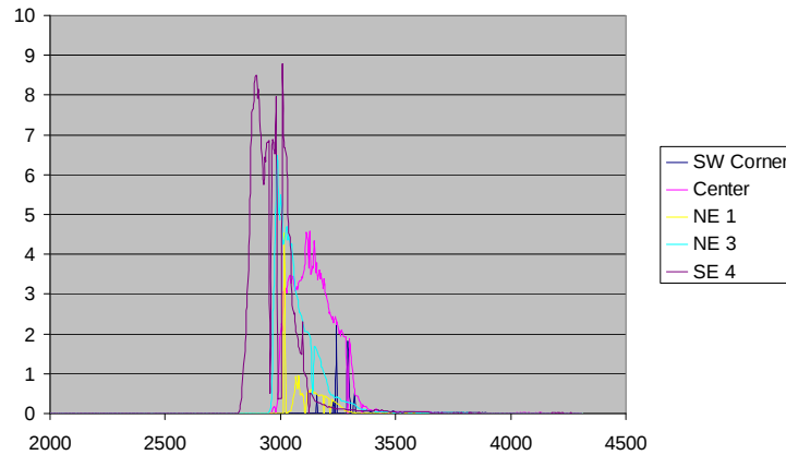
Figure 10. Example of LCD readings versus time for a 160 kg TEP release from southeast of the grid.
