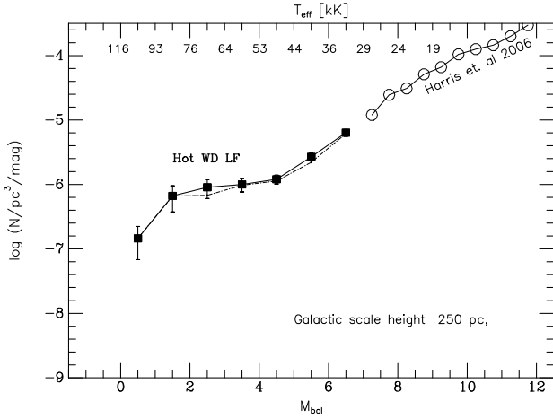
Fig. 4. Our WD LF as in Fig. 3, but with 1.0 mag bins.
