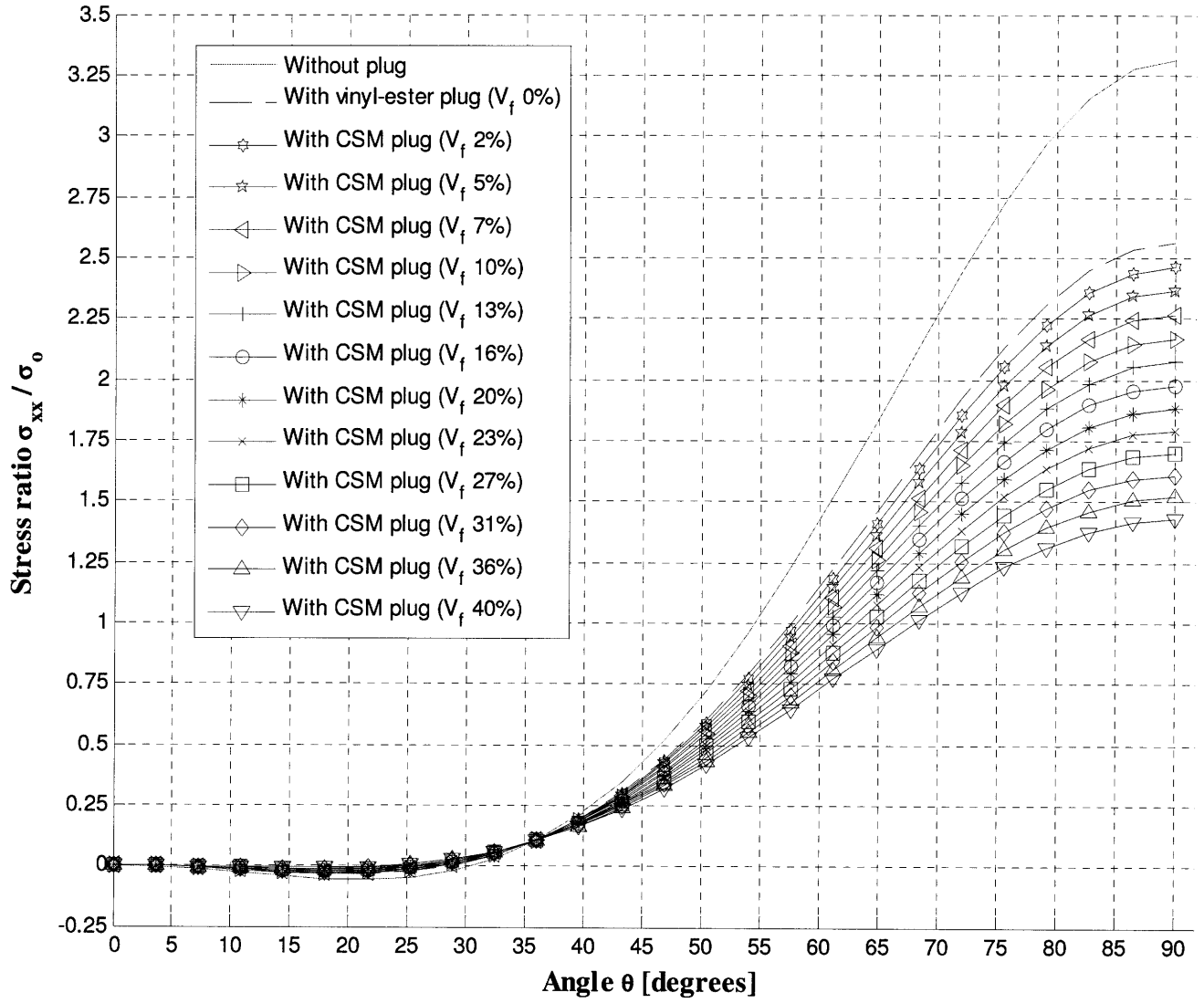
Figure C1: Stress \sigma_{xx} around hole in glass fiber / vinyl ester laminate of woven roving biased 60% in x -direction containing various plugs, and subjected to uniaxial tension \sigma_o in x -direction.
