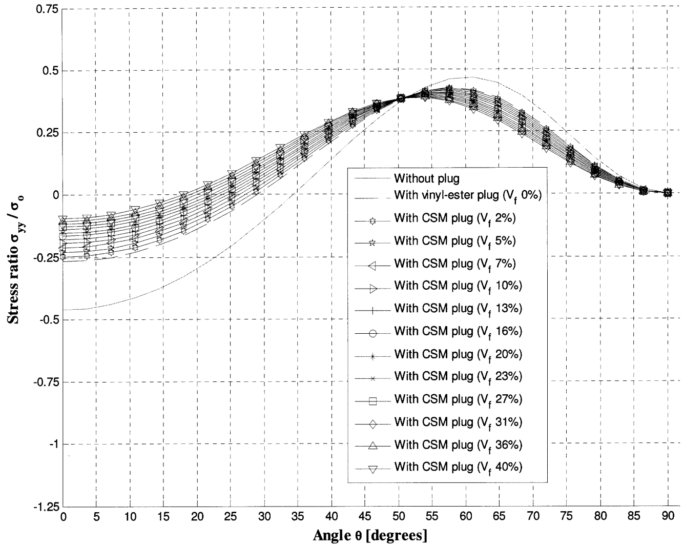
Figure C22: Stress \sigma_{yy} around hole in unidirectional glass fiber / vinyl ester laminate (aligned with x -direction) containing various plugs, and subjected to uniaxial tension \sigma_o in x -direction.
