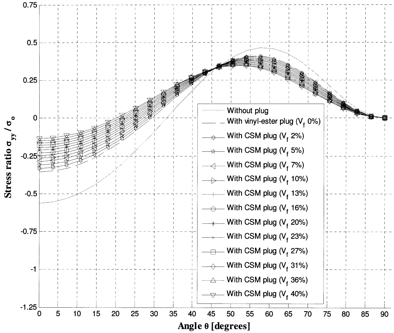
Figure C17: Stress \sigma_{yy} around hole in glass fiber / vinyl ester laminate of woven roving biased 90% in x -direction containing various plugs, and subjected to uniaxial tension \sigma_o in x -direction.
