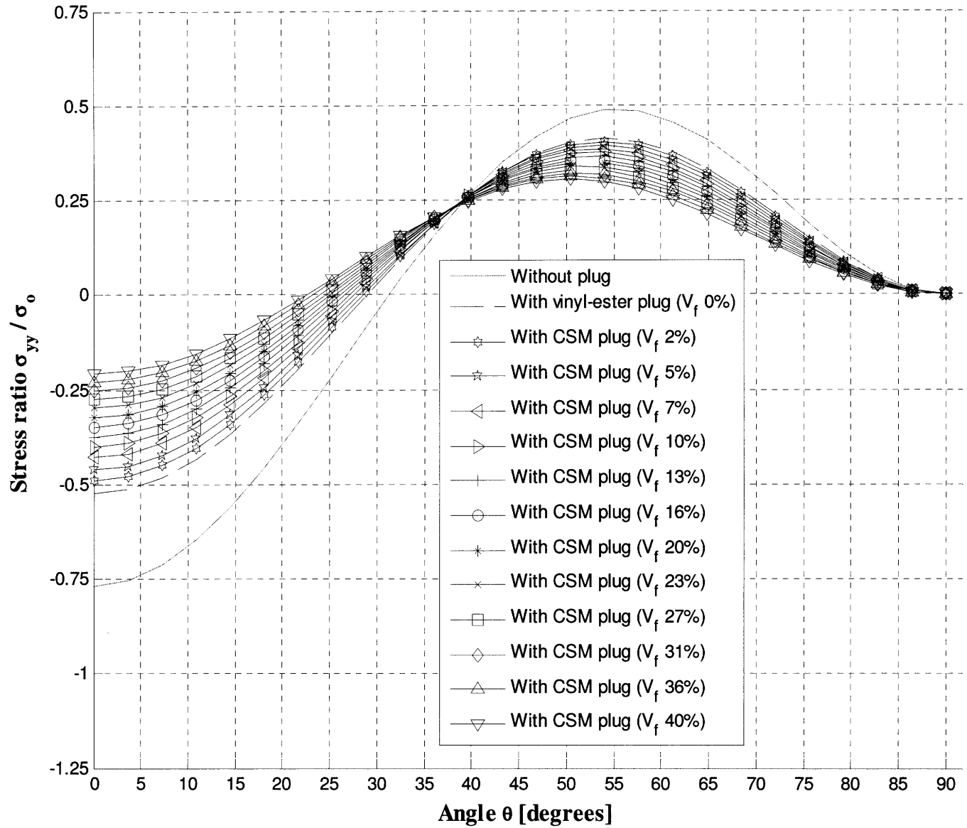
Figure C7: Stress \sigma_{yy} around hole in glass fiber / vinyl ester laminate of woven roving biased 70% in x -direction containing various plugs, and subjected to uniaxial tension \sigma_o in x -direction.
