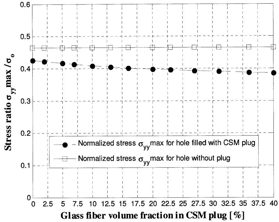
Figure C24: Normalized maximum stress \sigma_{yy} around edge of hole in unidirectional glass fiber / vinyl ester laminate (aligned with x -direction) for various chopped strand mat (CSM) plugs, and subjected to uniaxial tension \sigma_o in x -direction.
