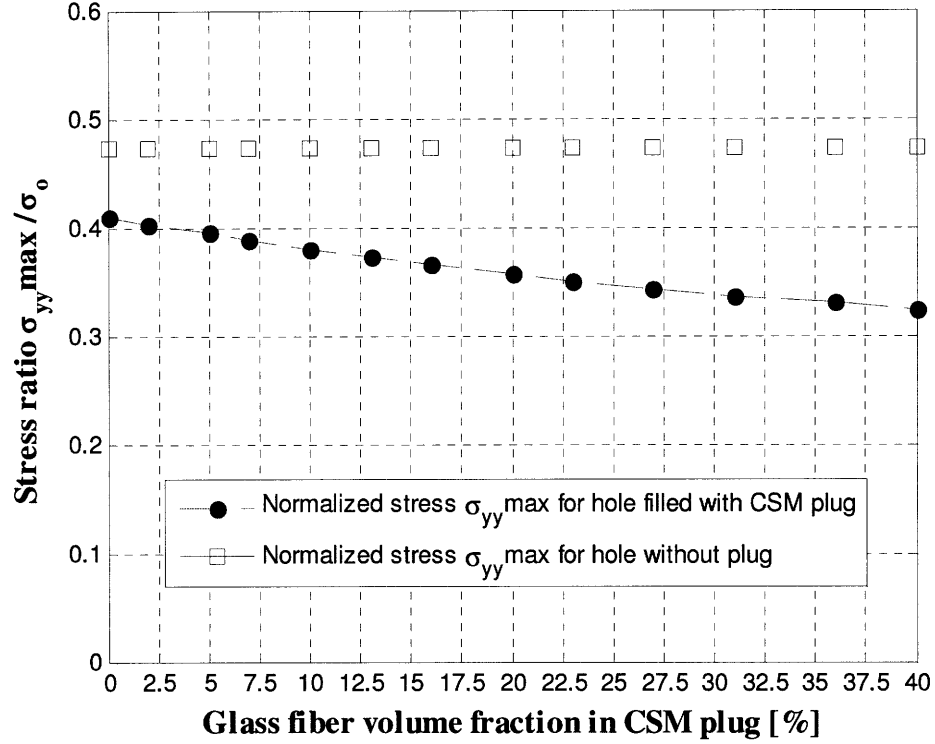
Figure C14: Normalized maximum stress \sigma_{yy} around edge of hole in laminate of glass fiber / vinyl ester woven roving (WR) biased 80% in x -direction for various chopped strand mat (CSM) plugs, and subjected to uniaxial tension \sigma_0 in x -direction.
