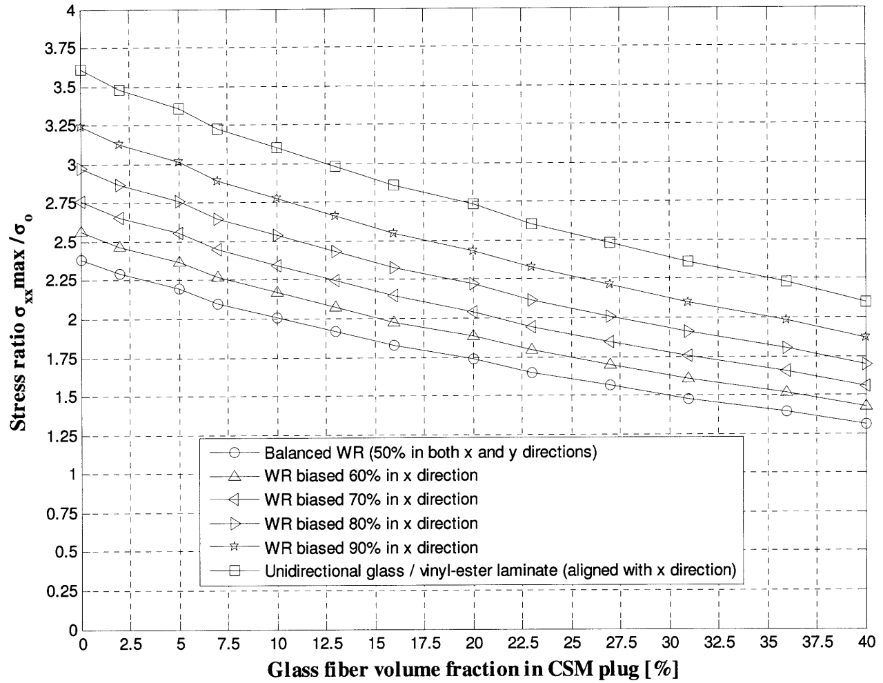
Figure 10: Normalized maximum stress \sigma_{xx} at hole in several laminates of woven roving (WR) for various chopped strand mat (CSM) plugs, subjected to uniaxial tension \sigma_o in x-direction.
