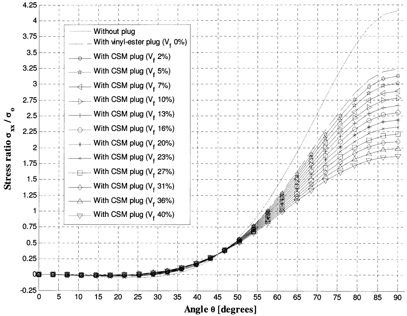
Figure C16: Stress \sigma_{xx} around hole in glass fiber / vinyl ester laminate of woven roving biased 90% in x-direction containing various plugs, and subjected to uniaxial tension \sigma_o in x-direction.
