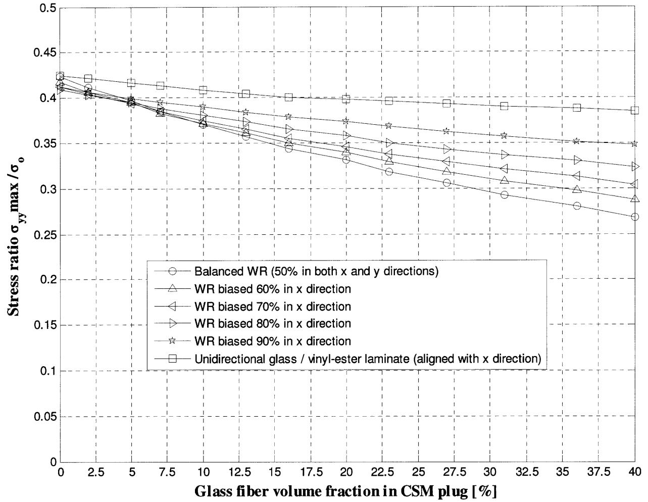
Figure 11: Normalized maximum stress \sigma_{yy} at hole in several laminates of woven roving (WR) for various chopped strand mat (CSM) plugs, subjected to uniaxial tension \sigma_o in x-direction.
