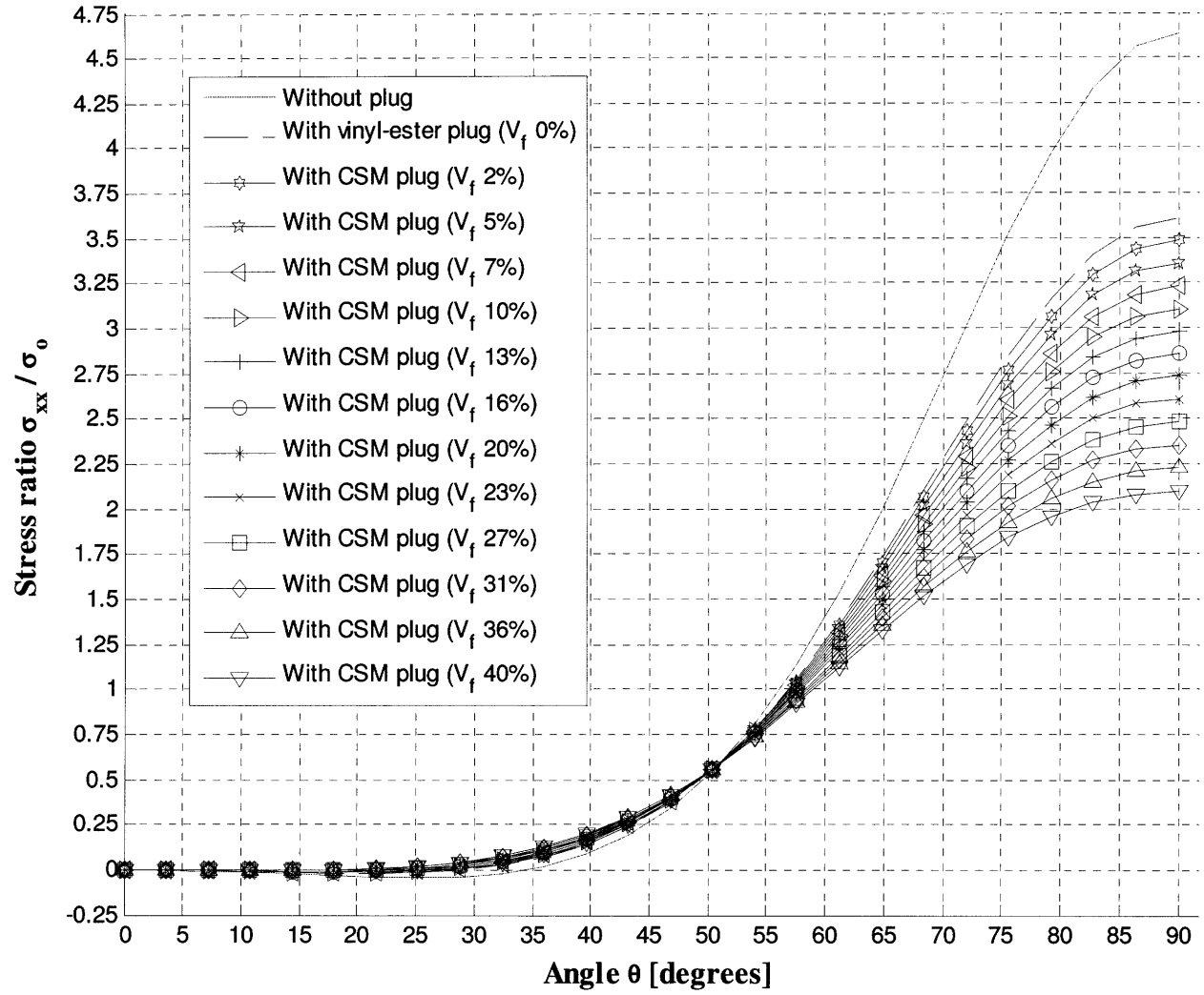
Figure C21: Stress \sigma_{xx} around hole in unidirectional glass fiber / vinyl ester laminate (aligned with x -direction) containing various plugs, and subjected to uniaxial tension \sigma_o in x -direction.
