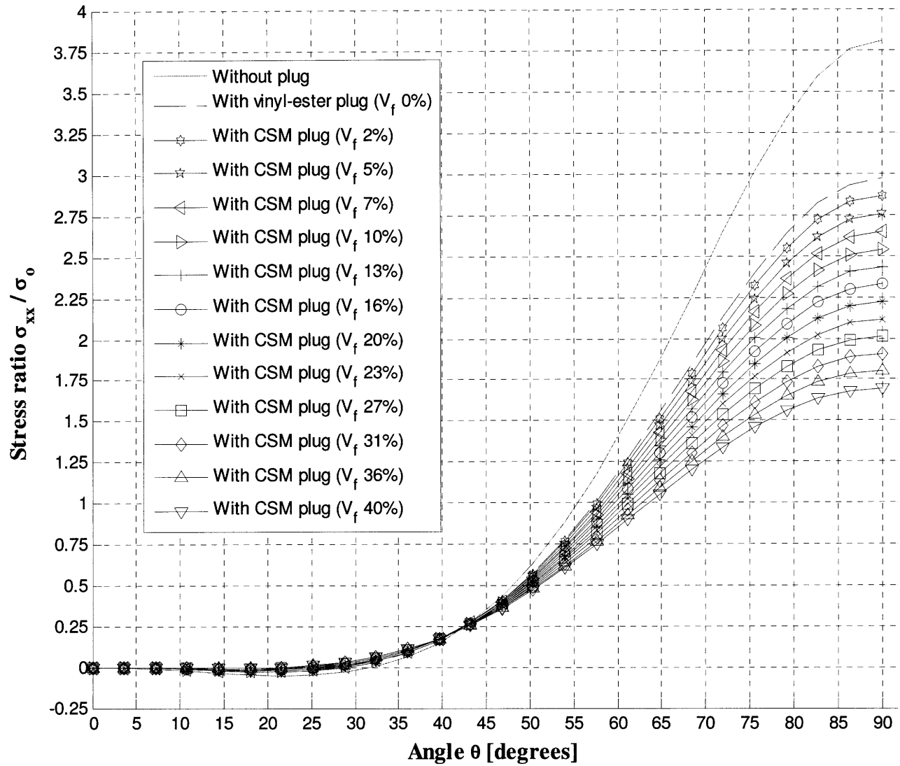
Figure C11: Stress \sigma_{xx} around hole in glass fiber / vinyl ester laminate of woven roving biased 80% in x-direction containing various plugs, and subjected to uniaxial tension \sigma_o in x-direction.
