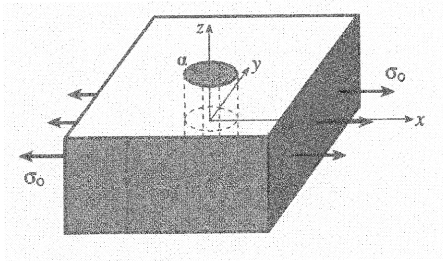
Figure 13: Schematic of three-dimensional plate with cylindrical hole under uniformly applied tensile stress.
