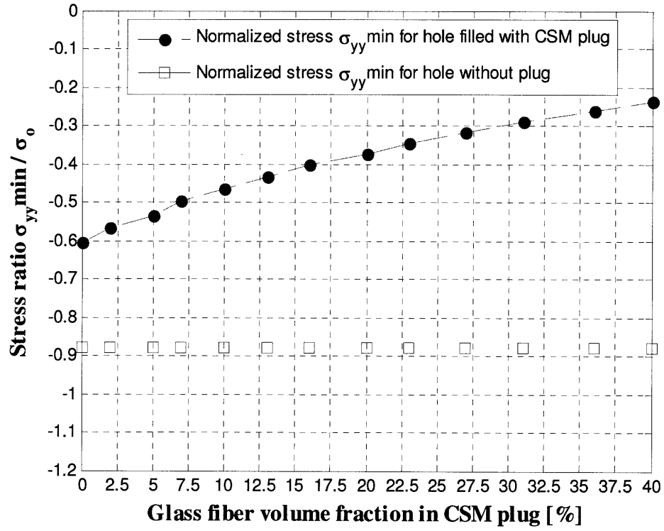
Figure C5: Normalized minimum stress \sigma_{yy} around edge of hole in laminate of glass fiber / vinyl ester woven roving (WR) biased 60% in x -direction for various chopped strand mat (CSM) plugs, and subjected to uniaxial tension \sigma_o in x -direction.
