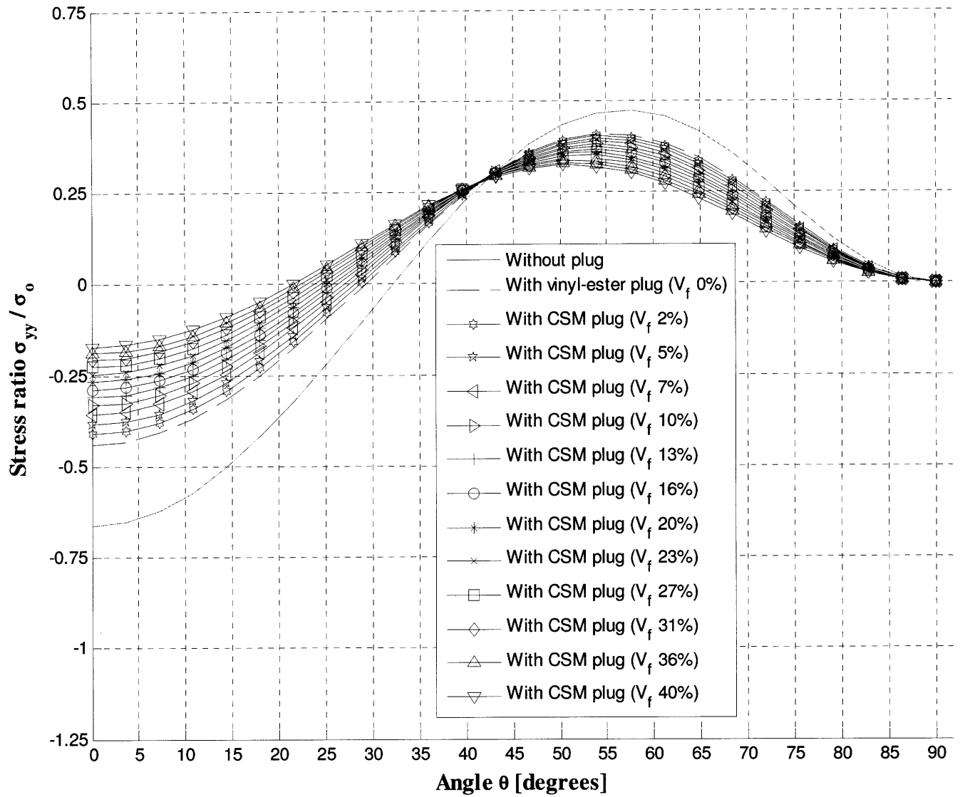
Figure C12: Stress \sigma_{yy} around hole in glass fiber / vinyl ester laminate of woven roving biased 80% in x-direction containing various plugs, and subjected to uniaxial tension \sigma_o in x-direction.
