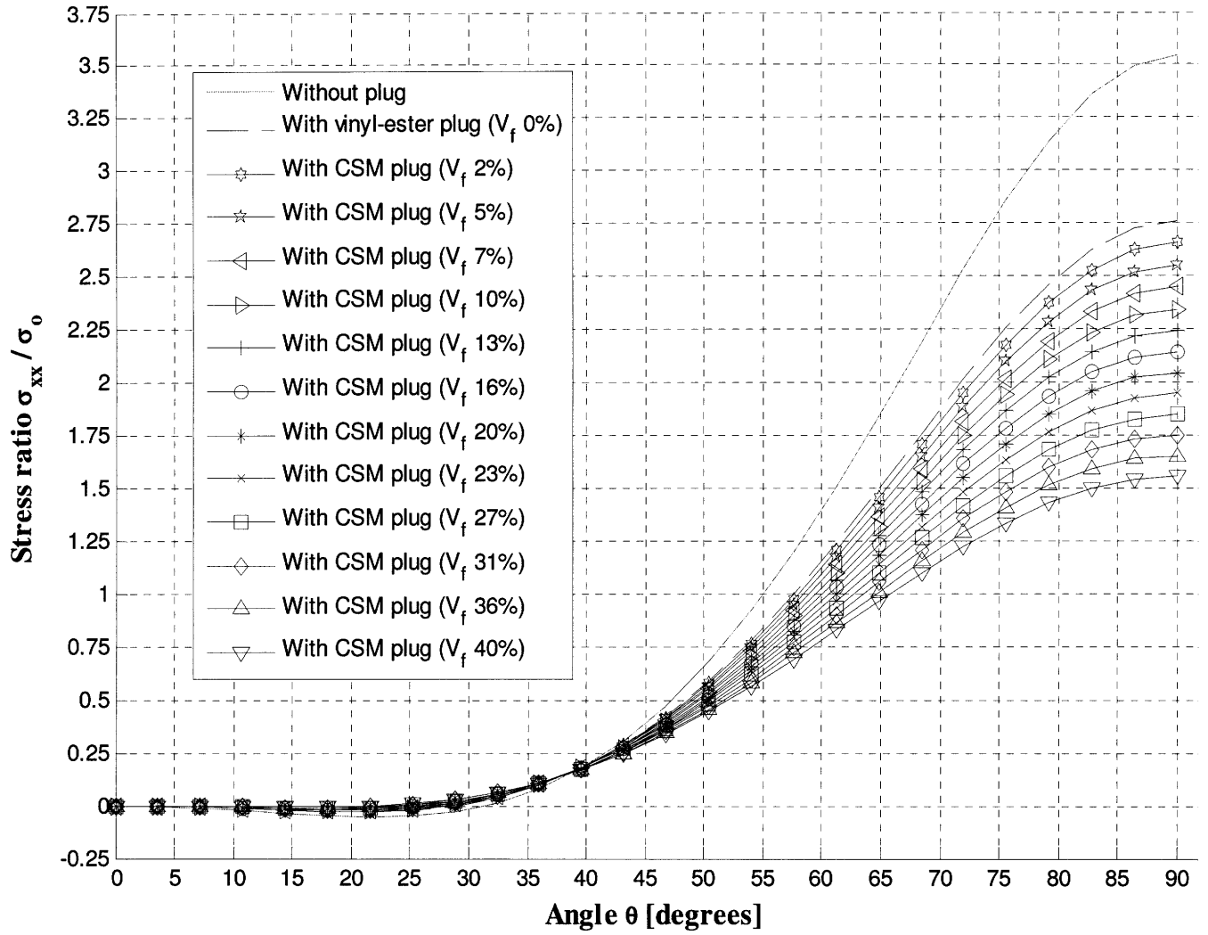
Figure C6: Stress \sigma_{xx} around hole in glass fiber / vinyl ester laminate of woven roving biased 70% in x -direction containing various plugs, and subjected to uniaxial tension \sigma_o in x -direction.
