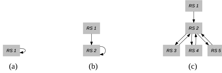
FIGURE 3.2: Static call graphs of three matrix-matrix multiplication libraries. We call the set that comprises all recursion steps of a given library the recursion step closure of the library. The first recursion step (RS1) captures the functionality that the user is interested in and is therefore part of the API (Application Program Interface): it is common to all libraries. However, the strategy to compute it is not fixed and, in particular, it can be decomposed into other recursion steps which are internal to the library. (a) is the naïve implementation and (b) is obtained after removing unnecessary explicit copies from it. Note that the closure can become more complicated, for instance (c) is obtained after an optimization to provide looped base cases.
