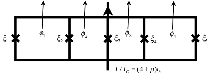
Figure 1. Four-Cell Array
