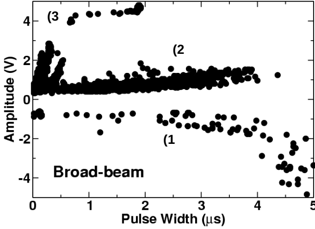
Fig. 10 Each point on the plots is representative of the amplitude vs. time-width at half maximum of amplitude (FWHM) of a SET observed at the output of the LM124 resulting from broad-beam experiments. The ions used during the experiment are 100MeV Br, 150 MeV Mg and 210 MeV Cl for angled strikes varying from 0^\circ to 60^\circ . The corresponding LETs values of the ions used are 38.6, 6.25 and 11.5 MeV.cm 2 /mg respectively.
