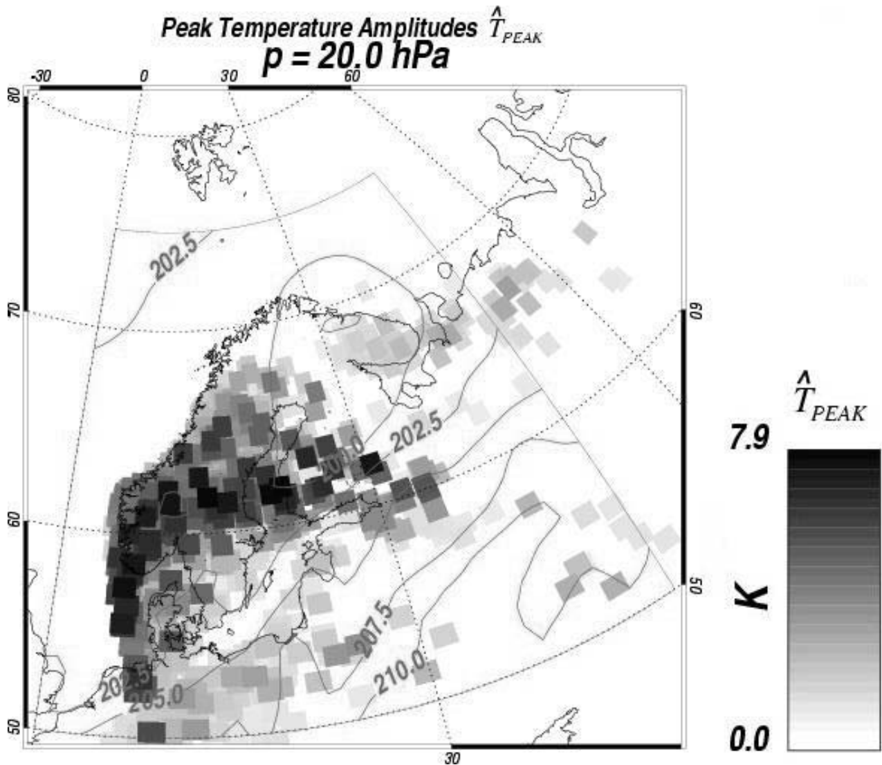
Figure 8. MWFM simulation of peak temperature amplitudes at 20 hPa on 2 March 2000, 0000 UT (colored squares). Each pixel represents the group location and amplitude of a ray. DAO analyzed background temperatures are represented as contours (labels in K). See color version of this figure at back of this issue.
