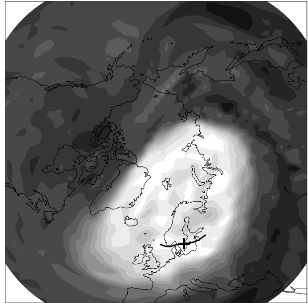
Figure 3. Potential vorticity (PV) on the 675 K isentropic surface on 2 March 2000 at 1200 UT from the ECMWF analysis. Darker areas correspond to low PV value (surge zone), while lighter areas correspond to high-PV values (polar vortex). The black cross, south of Sweden, indicates the position of the balloon at 1200 UT, and the balloon trajectory between 0600 and 1800 UT is also shown (bold curve).
