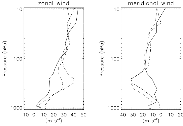
Figure 12. Zonal wind velocity (left) and meridional wind velocity (right) simulated by the ECMWF T319 model at 10°E, 58°N on 2 March 2000, at 0000 UT (solid), 0600 UT (dashed), and 1200 UT (dotted-dashed).
