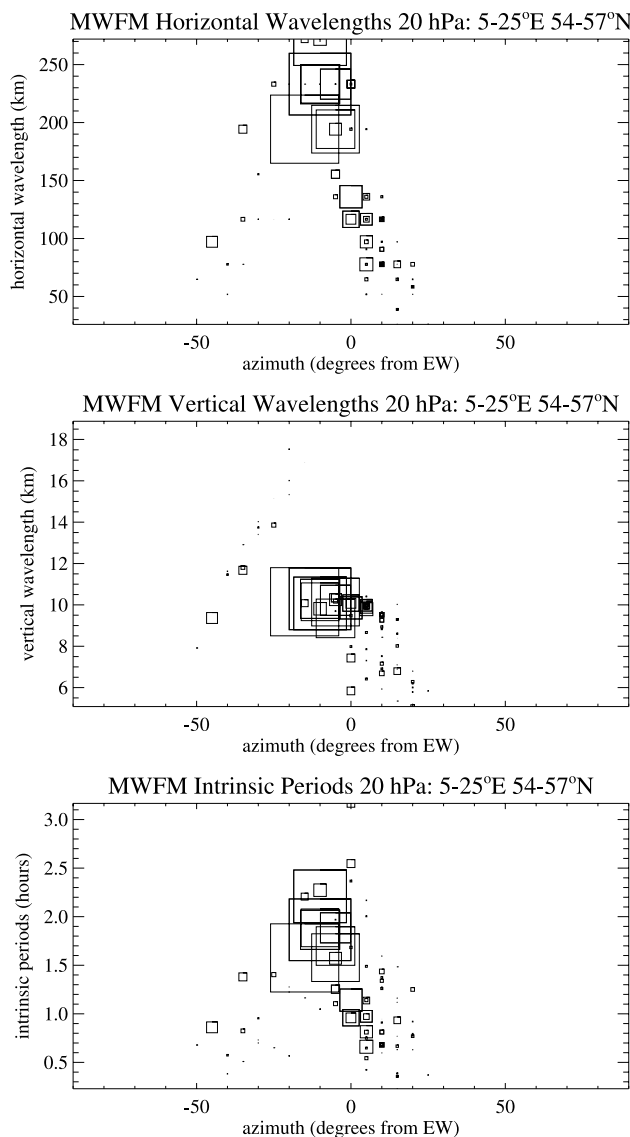
Figure 10. Scatterplots of horizontal wavelengths (upper panel), vertical wavelengths (middle panel), and intrinsic periods (lower panel) of rays simulated by the MWFM model above southern Scandinavia. The size of the symbols is proportional to the square of the temperature fluctuations associated with each ray.
