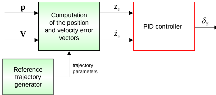
Figure 13 Vertical channel tracking controller structure
