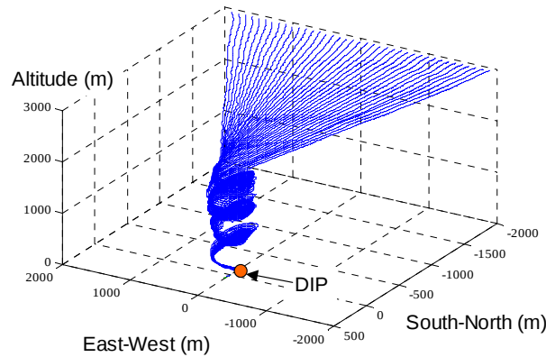
Figure 15 Simulation results of the trajectory tracking control system
