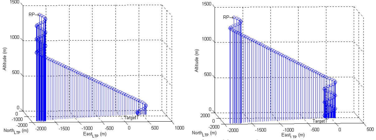
Figure 5 3D representation of possible inertial RTs
