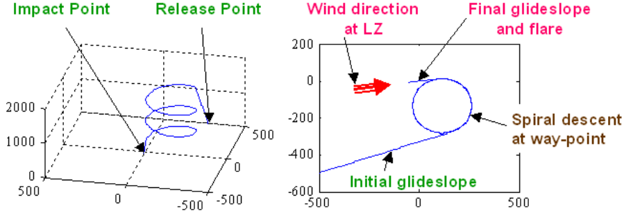
Figure 7 Graphical representation of the parafoil trajectory
