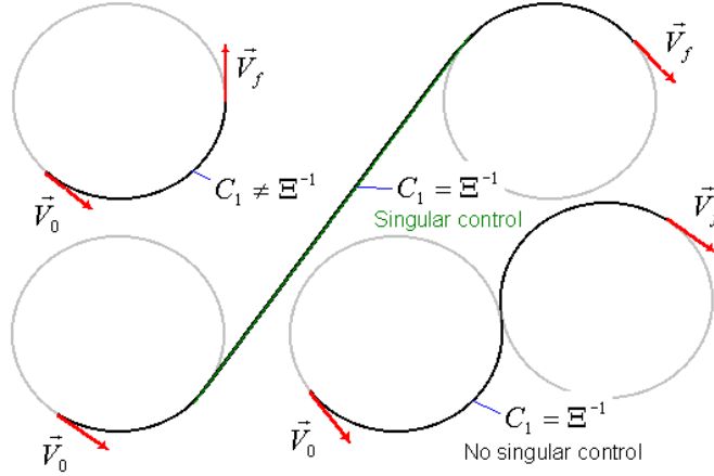
Figure 4 Planar projections of possible trajectories
