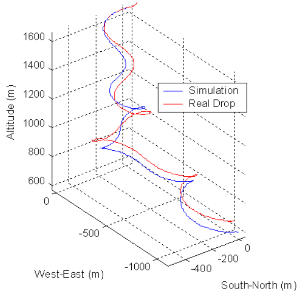
Figure 14 Comparison of the flight test data and simulation results
