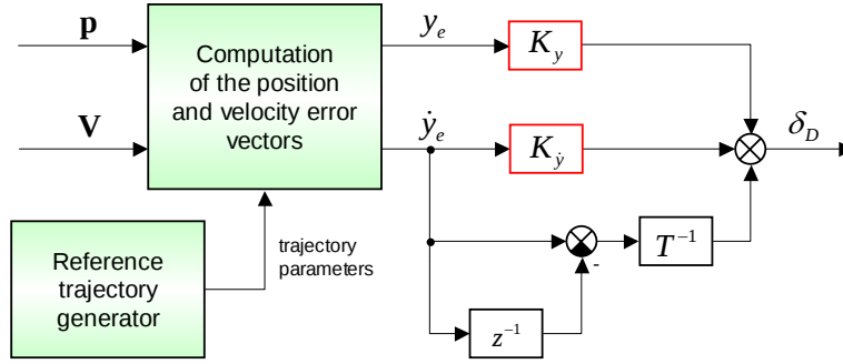
Figure 12 Lateral channel tracking controller structure
