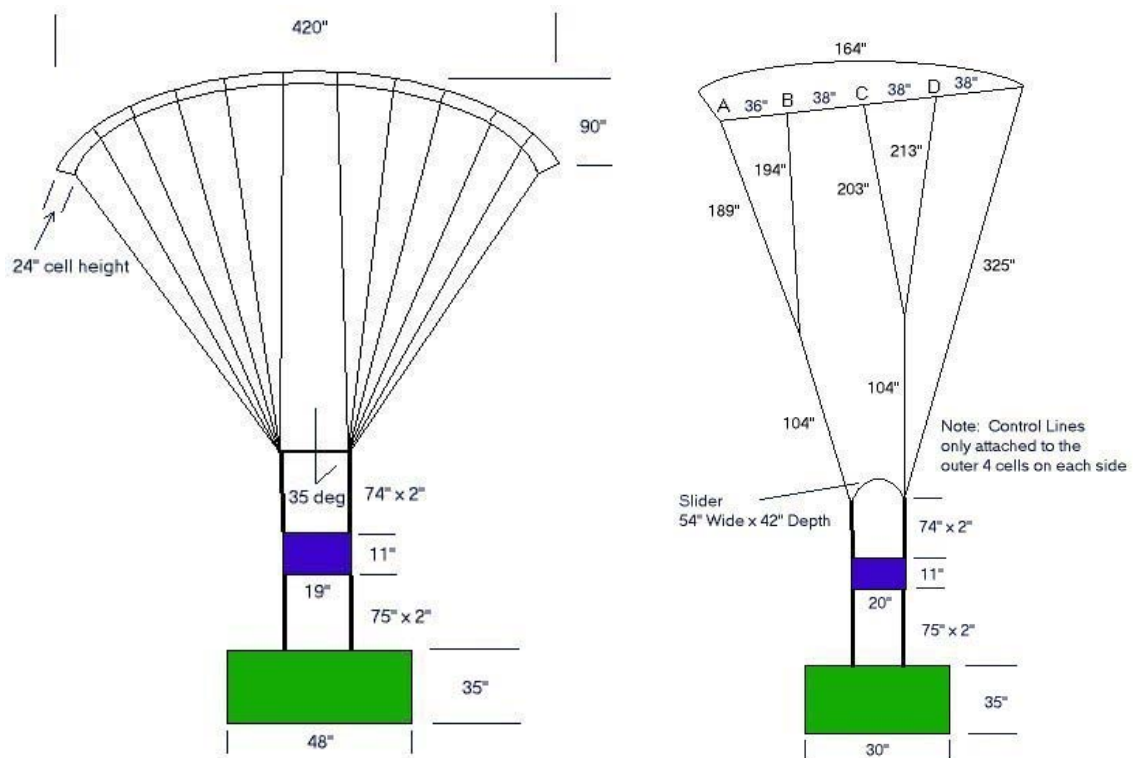
Figure 3 The 500lb parafoil geometry
