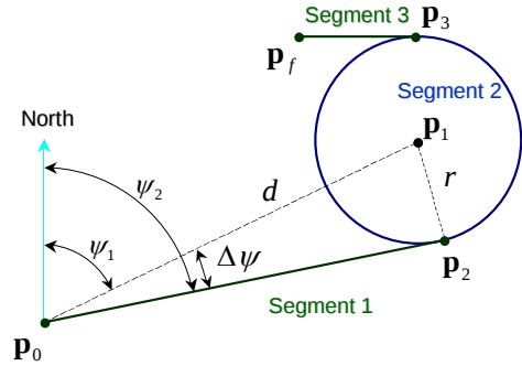
Figure 8 Top view of the parafoil RT
