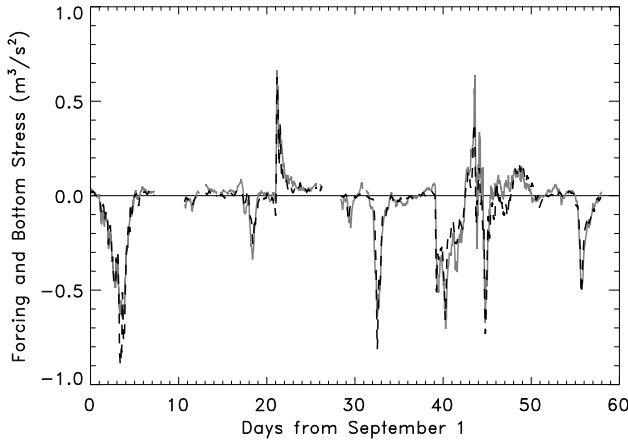
Figure 7. Hourly total forcing (wind and wave, -S_{yx}/\rho|_{x_{8m}} + \int_0^{x_{8m}} (\tau_y^{\text{wind}}/\rho) dx , solid curve) and bottom stress ( c_f \int_0^{x_{8m}} \langle |\vec{u}|v \rangle dx , dashed curve) integrated from the shoreline to 8-m depth with a best fit c_f = 0.0015 versus time. Gaps occur when the bottom stress integral could not be computed because of inactive sensors. The correlation coefficient squared r^2 = 0.87 .
