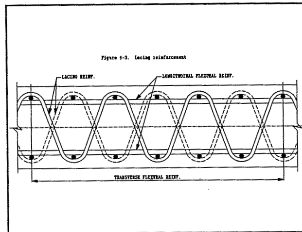
Figure 1. Illustration of lacing reinforcement (Fig. 4-3, Ref. 1)
