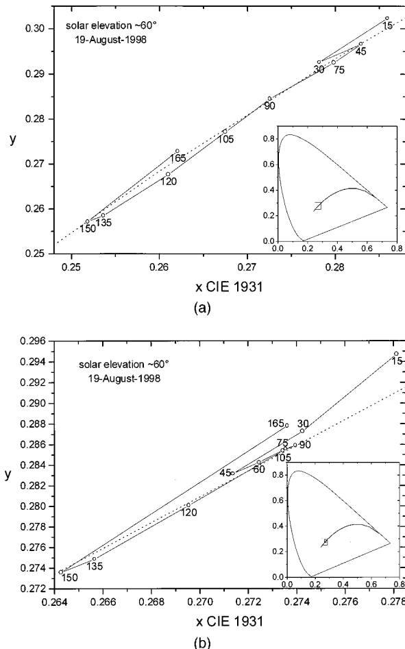
Fig. 4. (a) Chromaticity curve for Granada clear skylight along \phi_{\text{rel}} = 0^\circ (the clear-sky principal plane) when solar elevation h_0 = 60^\circ on August 19, 1998. Note that view elevations beyond the zenith are indicated by h > 90^\circ . The dotted line is the CIE daylight locus, while the inset shows the entire CIE 1931 diagram and Planckian locus. Figures 5–7 reuse Fig. 4's notation. (b) Chromaticity curve for clear skylight along \phi_{\text{rel}} = 90^\circ when h_0 = 60^\circ (August 19, 1998).
