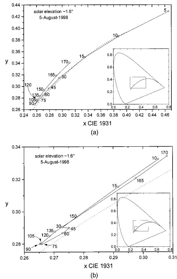
Fig. 7. (a) Chromaticity curve for clear skylight along \phi_{\text{rel}} = 0^\circ when h_0 = 1.6^\circ (August 5, 1998). (b) Chromaticity curve for clear skylight along \phi_{\text{rel}} = 90^\circ when h_0 = 1.6^\circ (August 5, 1998).
