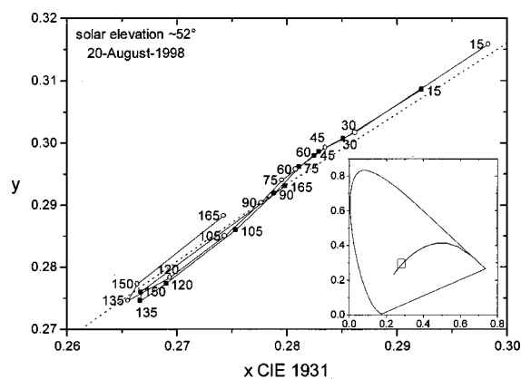
Fig. 10. Chromaticity curves for Granada clear skylight along \phi_{\text{rel}} = 45^\circ, 315^\circ when h_0 = 52^\circ (August 20, 1998).
