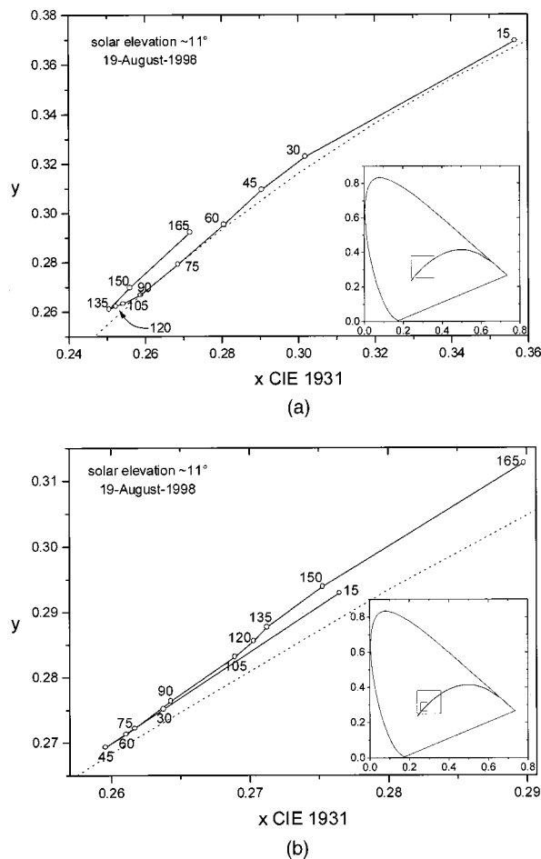
Fig. 6. (a) Chromaticity curve for clear skylight along \phi_{\text{rel}} = 0^\circ when h_0 = 11^\circ (August 19, 1998). (b) Chromaticity curve for clear skylight along \phi_{\text{rel}} = 90^\circ when h_0 = 11^\circ (August 19, 1998).
