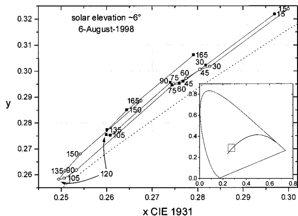
Fig. 12. Chromaticity curves for Granada clear skylight along \phi_{\text{rel}} = 45^\circ, 315^\circ when h_0 = 6^\circ (August 6, 1998).
