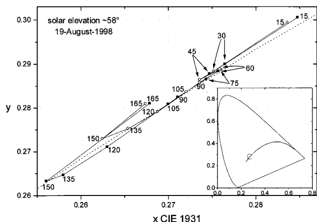
Fig. 9. Chromaticity curves for Granada clear skylight along \phi_{\text{rel}} = 45^\circ, 315^\circ when solar elevation h_0 = 58^\circ on August 19, 1998. Chromaticities along \phi_{\text{rel}} = 45^\circ are denoted with filled squares; those along \phi_{\text{rel}} = 315^\circ , with open circles. As in Figs. 4–7, view elevations beyond the zenith at each \phi_{\text{rel}} are indicated by h > 90^\circ . The dotted line is the CIE daylight locus, while the inset shows the entire CIE 1931 diagram and Planckian locus. Figures 10–12 reuse Fig. 9's notation.
