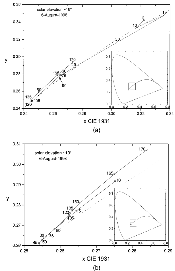
Fig. 5. (a) Chromaticity curve for clear skylight along \phi_{\text{rel}} = 0^\circ when h_0 = 19^\circ (August 6, 1998). (b) Chromaticity curve for clear skylight along \phi_{\text{rel}} = 90^\circ when h_0 = 19^\circ (August 6, 1998).
