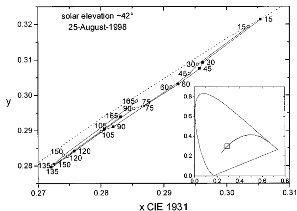
Fig. 11. Chromaticity curves for Granada clear skylight along \phi_{\text{rel}} = 45^\circ, 315^\circ when h_0 = 42^\circ (August 25, 1998).
