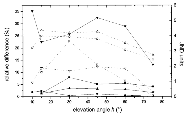
Fig. 8. Relative luminance differences (solid symbols) and chromaticity differences in JND units (open symbols) as a function of h along \phi_{\text{rel}} = 90^\circ for the four h_0 shown in Figs. 4(b), 5(b), 6(b), and 7(b). Solar elevation symbols are squares for h_0 = 60^\circ , circles for h_0 = 18.5^\circ , upright triangles for h_0 = 10^\circ , and inverted triangles for h_0 = 0.4^\circ .
