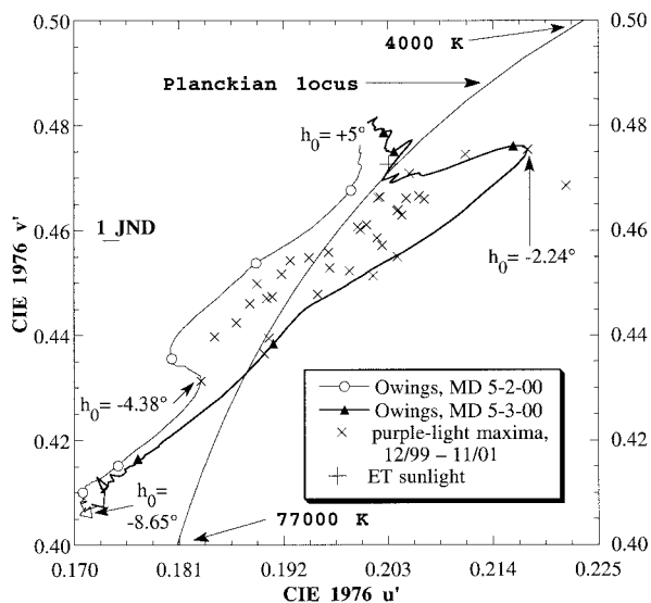
Fig. 11. Variability of 35 purple-light maxima at three of our observing sites. Complete temporal chromaticity curves are drawn for Owings, Maryland, on 2–3 May 2000, two adjacent days with the largest colorimetric difference in purple-light maxima measured from December 1999 to November 2001.
