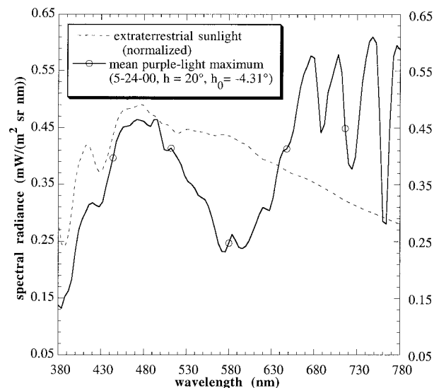
Fig. 12. Visible-wavelength spectral radiance for a typical purple-light maximum measured at Owings on 24 May 2000 when h_0 = -4.31^\circ compared with those of sunlight above the atmosphere (normalized to have the same sum as the purple-light spectrum). Of the 35 purple-light maxima plotted in Fig. 11, this purple-light spectrum has the chromaticity that is closest to the mean u', v' .
