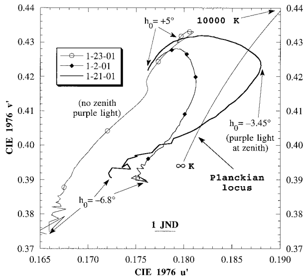
Fig. 8. Temporal trends in evening twilight chromaticities measured at the zenith at Owings, Maryland, on 2, 21, and 23 January 2001. Although the 21 January twilight has a distinct purple light, two days later there is none.
