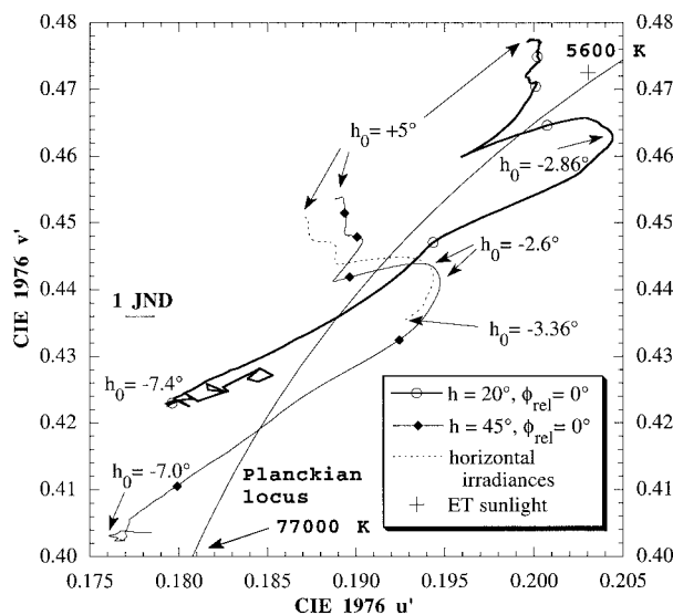
Fig. 9. Temporal trends in evening purple-light chromaticities at Granada, Spain, on 7 June 2000 for horizontal daylight irradiances and for skylight radiances at h = 20^\circ, 45^\circ and \phi_{\text{rel}} = 0^\circ .
