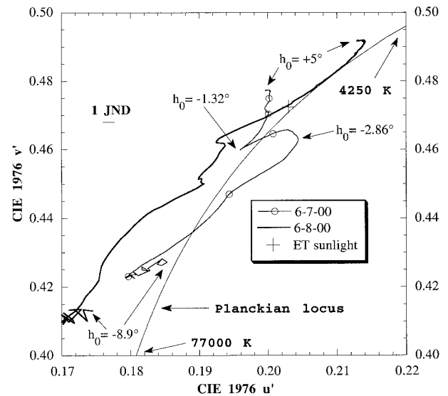
Fig. 10. Comparison of temporal trends in evening twilight chromaticities at Granada on 7-8 June 2000 ( h = 20^\circ, \phi_{\text{rel}} = 0^\circ ). Note that the vivid purple light of 7 June largely disappears by the next day.
