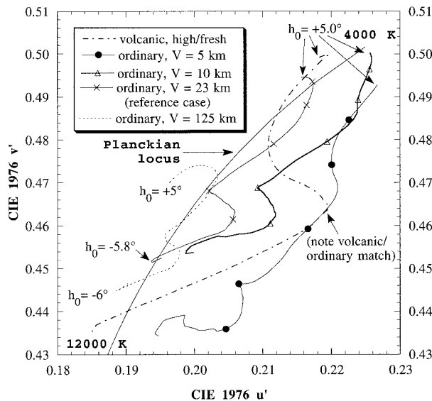
Fig. 17. Radiative transfer model LOWTRAN 7's calculations of temporal chromaticity trends for ordinary purple light as functions of h_0 and meteorological range V at h = 20^\circ and \phi_{\text{rel}} = 0^\circ . For comparison, we also show a chromaticity curve calculated for a volcanic twilight with high levels of fresh volcanic scatterers in the stratosphere. Note the similarities between the V = 23 km curve (our LOWTRAN reference case) and the purple-light chromaticities measured in Figs. 5 and 13.
