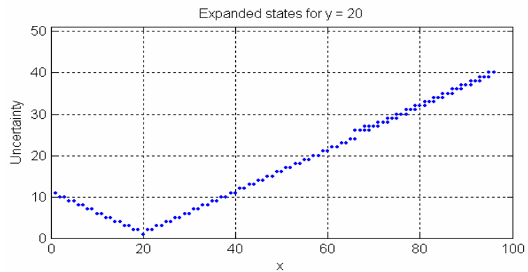
Figure 17. State expansion for binary cost world
