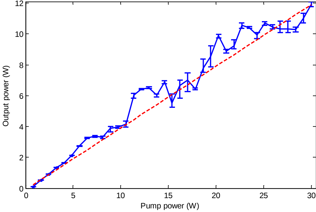
Figure 30: Output power vs incident pump power for single-leg Z-cavity. The average slope efficiency is \sim 40\% . The error bars show the minimum and maximum of 1000 measurements of output power per second at each data point. The output power oscillation and random non-linearity of the curve are attributed to thermal lensing instability and the random pump beam distortions caused by atmospheric water vapor absorption of the pump radiation.
