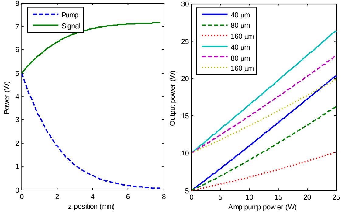
Figure 28: Example model predictions showing (left) input signal growth and pump absorption over the crystal length for 5 W input signal and 5 W pump, both at 80 \mu\text{m} spot size and (right) amplification comparisons for 5 and 10 W input signal powers with varying spot size as a function of pump power.
