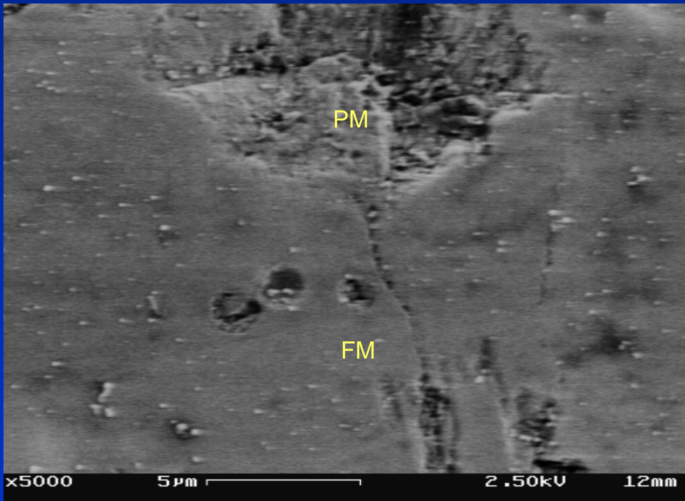
Partially-molten domain with \alpha -Al 2 O 3 grains stops the crack propagating from the bottom
