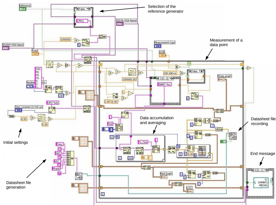
Fig. 6. Block-diagram of the LabVIEW tool for automation of the fluorescence lifetime measurements in the frequency domain.
