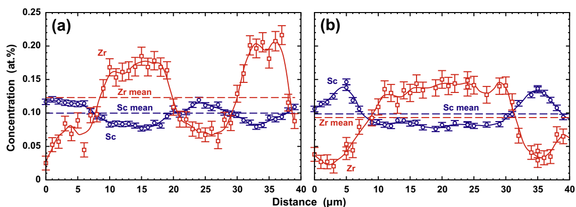
Fig. 2. Concentration profiles of Sc and Zr, measured by EPMA, across multiple dendritic cells from two regions in as-cast Al-0.1Sc-0.1Zr(a). The horizontal dashed lines indicate the mean measured solute concentrations.
