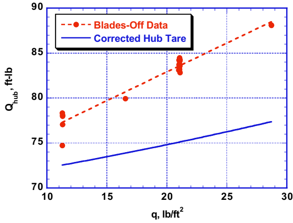
Fig. 10. Effect of dynamic pressure on hub torque tare, \alpha = 0 \text{ deg} .
