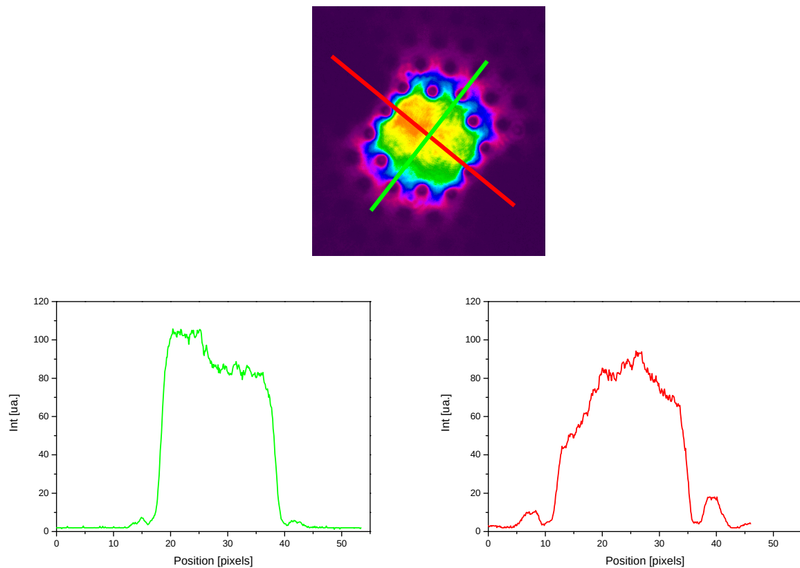
Figure 19 Mode profiles at 1060 nm in the two orthogonal directions (indicated by the colour)
