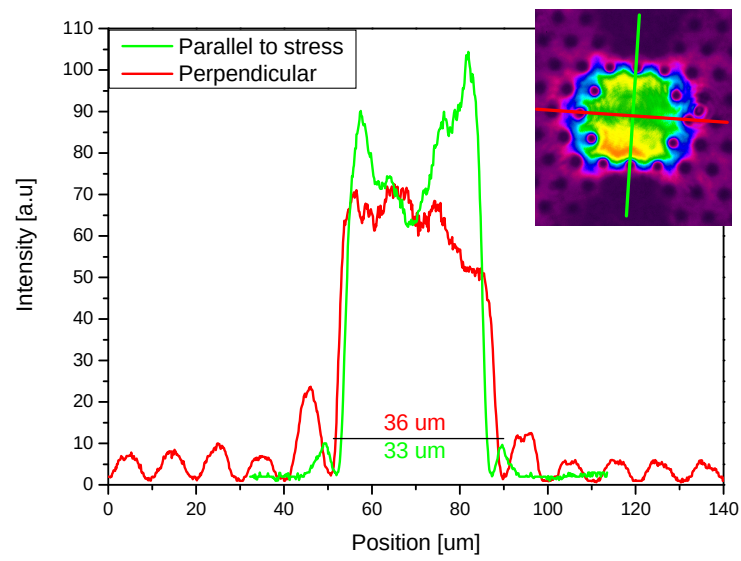
Figure 15 Mode profile (measured at 1060 nm) of Fiber 4 bend to \sim 130 cm diameter.
