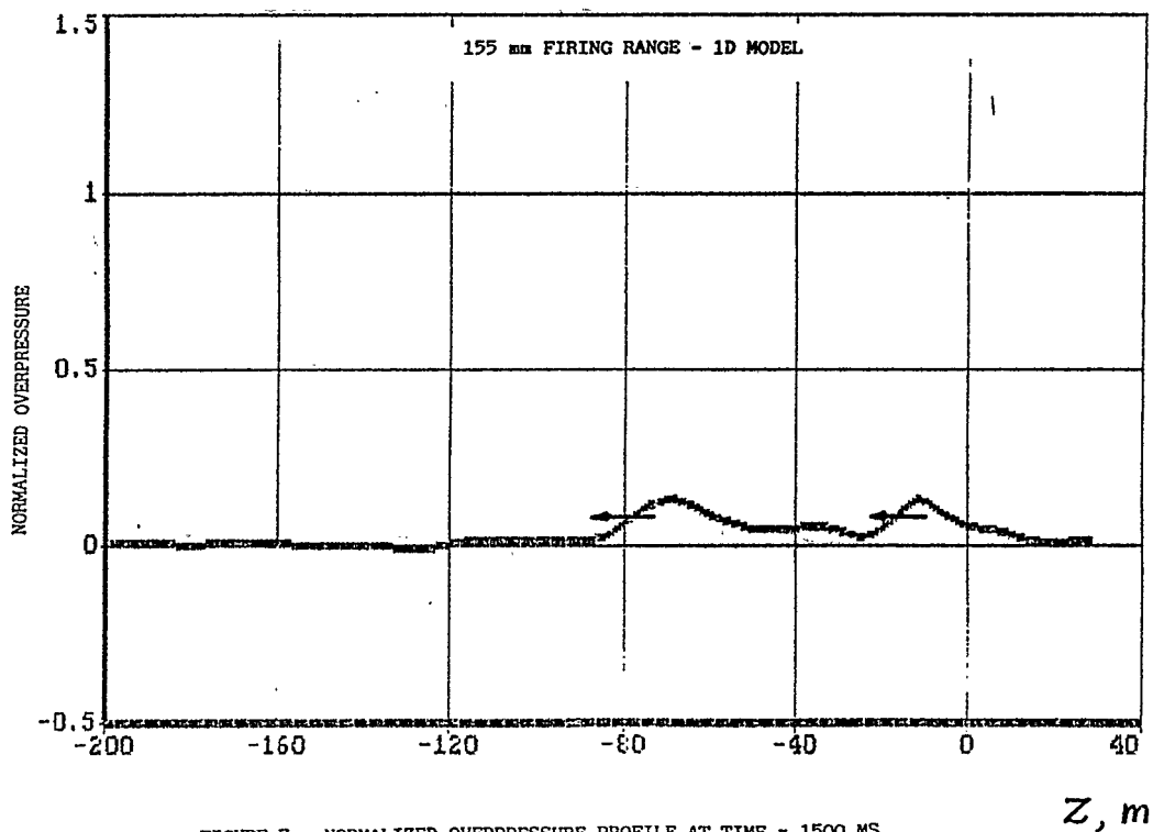
FIGURE 7: NORMALIZED OVERPRESSURE PROFILE AT TIME = 1500 MS. (UNIFORM CROSS-SECTION RANGE).
