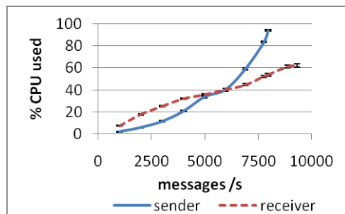
Figure 16. Processor utilization as a function of the multicast rate (100 receivers).
