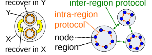
Figure 7. Hierarchical recovery in QSM (left) applied to topics vs. regions (right).
