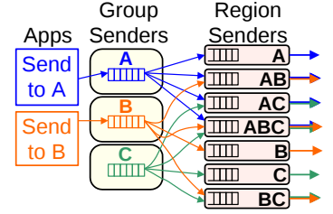
Figure 6. A message targeted at a topic is transmitted to all regions that topic spans over.
