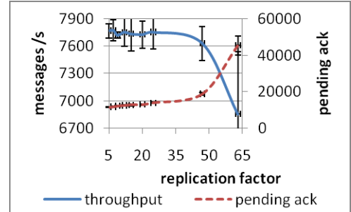
Figure 27. As the number of caching replicas increases, the throughput decreases.
