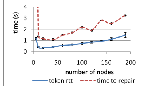
Figure 32. Token roundtrip time and the time to recover in the "sleep" scenario.
