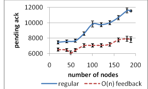
Figure 23. More aggressive cleanup with O(n) feedback in the token and in ACKs.
