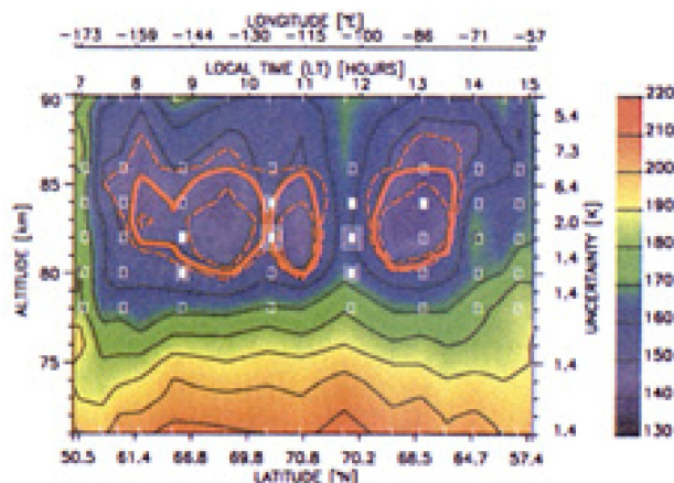
Figure 3. CRISTA temperatures measured on August 14 between 18.5 and 18.8 UT. The path described by latitude, longitude, and local time is the same as that by the outlined squares in Figure 2 and is referenced to an 82.0 km tangent altitude. The solid red contour is the frost point calculated using water vapor inferred from MAHRSI OH observations. Open symbols show a MAHRSI limb observation where the area subtended at the tangent altitude by the slit is approximately to scale. Solid symbols show a PMC detection with a background brightness of 1.2–2 times the clear air result, one box around the symbol is 2–4 times clear air conditions, and two boxes indicate the observation is 4–6 times clear air. CRISTA scan locations over which the image is interpolated are shown by tick marks on the inside border of the image and uncertainties are indicated on the right hand axis.
