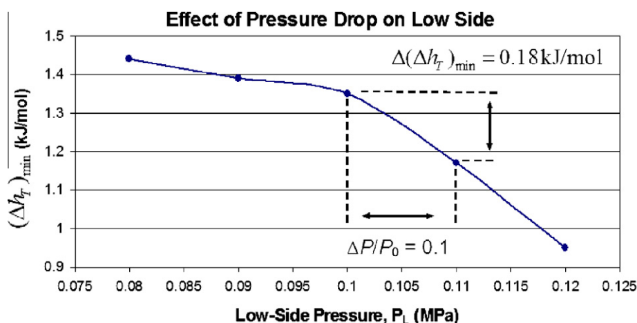
Fig. 4. Effect of pressure drop in the low-side on the minimum enthalpy difference. As shown, a 10% pressure increase on the low-side due to a pressure drop causes 0.18 kJ/mol loss in enthalpy difference.
