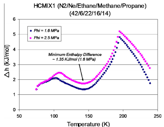
Fig. 2. Enthalpy difference vs. temperature of an optimized five-component mixed refrigerant. Both enthalpy difference of 0.1 MPa (1 bar)–1.6 MPa (16 bar) and 0.1 MPa (1 bar)–2.5 MPa (25 bar) are plotted as a function of temperature.
