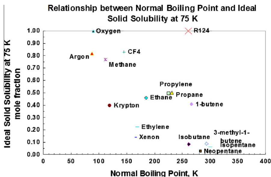
Fig. 3. Ideal solid solubility at 75 K of commonly used components in mixtures as a function of their normal boiling points.
