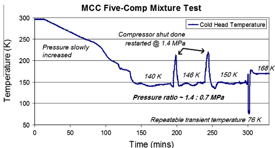
Fig. 5. Cooling test of the MCC using five-component mixed refrigerant. The mixture is precooled to 240 K before sending into the MCC, and the cold head temperature is measured by a thin film Ti thermometer affixed on it.
