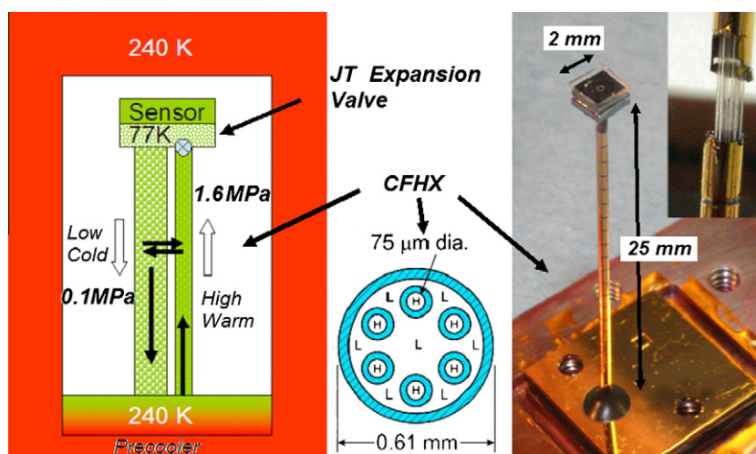
Fig. 1. Schematics and photos of the MCC. The left schematic illustrates the MCC key components, which are the JT expansion valve, the CFHX, and the precooler. High pressure warm gas is pumped through the fibers (as shown in cross sectional views) in the CFHX to the JT expansion valve. The expanded cooled gas returns back in the interstitial spaces in the CFHX to precool the incoming gas. The direction of flow is indicated with arrows. Photos of the MCC assembly and fibers in the capillary are shown on the right hand side.
