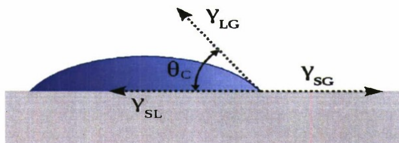
Figure 14 Surface tension by contact angle diagram
