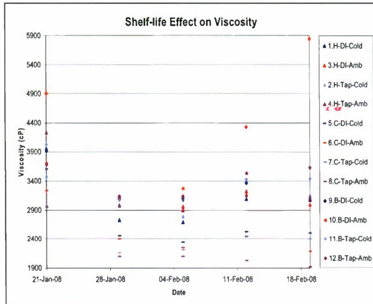
Figure 24 Shelf-life viscosity
