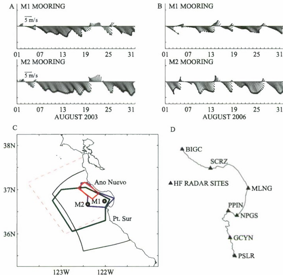
Figure 1. Observed wind velocities at M1 and M2 during (a) August 2003 and (b) August 2006. (c) M1 and M2 moorings locations, the NCOM ICON model domain (bounded by solid black line), areas sampled by Slocum (bounded by blue line) and Spray (bounded by green line) gliders in August 2003, the area sampled by gliders in August 2006 (bounded by solid red line), and the area of cruise surveys (bounded by dashed red line) are shown. (d) Locations of HF radar sites are shown.
