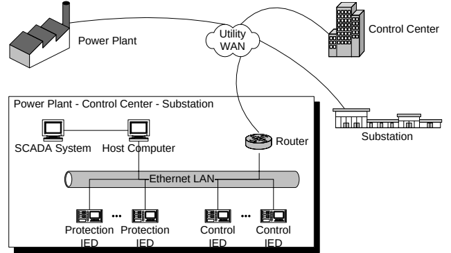
Fig. 2. Placement of the Agent-based IEDs within the Utility Intranet
