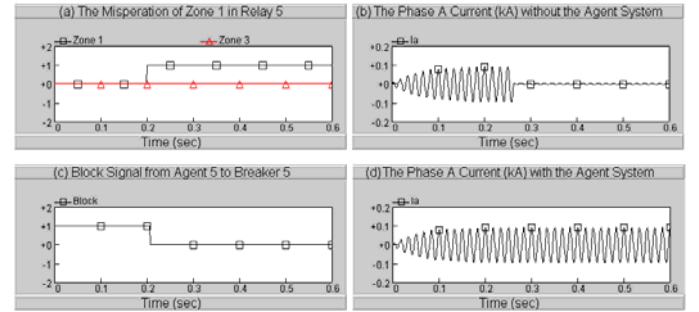
Fig. 6: (a) A primary relay misoperates at time 0.2 by setting a trip signal. (b) A traditional backup protection system would allow the breaker to trip, cutting power across the line. (c) The agent-based protection system communicates with its neighbors and determines that the trip signal should be blocked. (d) The agent-based system blocks the false trip signal.
