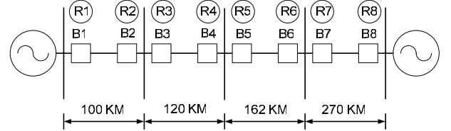
Fig. 5. A 400 kV power system with an agent-based backup protection system.
