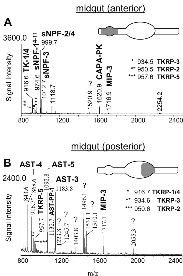
Figure 8. MALDI-TOF mass spectra of preparations of midgut tissue from freshly hatched male Ae. aegypti ; which demonstrate the uneven distribution of a number of neuropeptides in the midgut. (A) Preparation of an anterior portion of the midgut. (B) Preparation of a posterior portion of the midgut. AST, allatostatin; TKRP, tachykinin-related peptide; sNPF, short neuropeptide F, MIP, myoinhibitory peptide; PK, pyrokinin.
