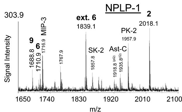
Figure 4. MALDI-TOF mass spectrum of a preparation of the tritocerebrum demonstrating the abundance of the C-terminal extended NPLP-1-6 in comparison to the predicted NPLP-1-6 sequence (for better visibility only a limited mass range of 1650–2100 is shown). The NPLP-1 peptides are designated with numbers. SK, sulfakinin; PK, pyrokinin; AST, allatostatin.
