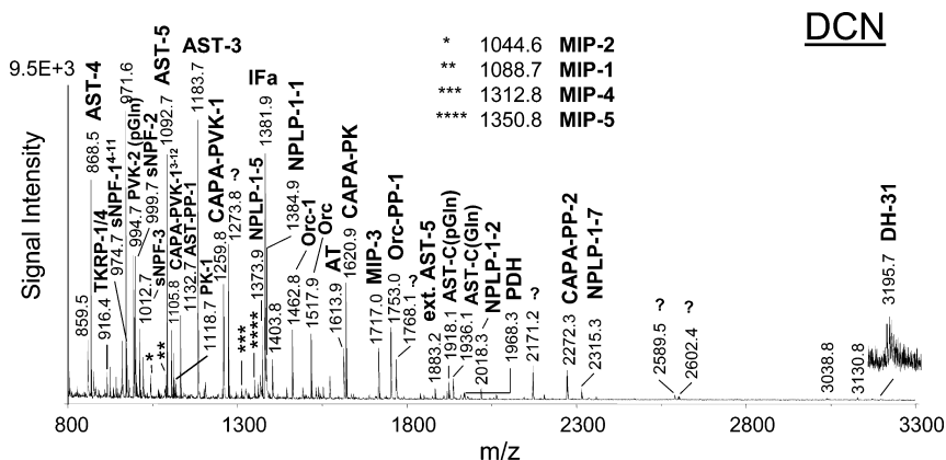
Figure 5. MALDI-TOF mass spectrum of a preparation of the dorso-caudal neuropil (DCN) of the terminal ganglion. The number of different neuropeptides in the DCN of Ae. aegypti was not surpassed by any other distinct region of the CNS; in this spectrum, mature products of 12 neuropeptide precursors are detectable (due to shortage of space, not all neuropeptide signals are designated). The question marks designate putative peptides which could not be assigned to the neuropeptide precursors of Ae. aegypti . PK, pyrokinin; AST, allatostatin; TKRP, tachykinin-related peptide; sNPF, short neuro peptide F, PVK-periviscerokin; NPLP, neuro peptide-like precursor; Orc, orcokinin; AT, allatotropin; MIP, myoinhibitory peptide; PDH, pigment dispersing hormone; DH, diuretic hormone.
