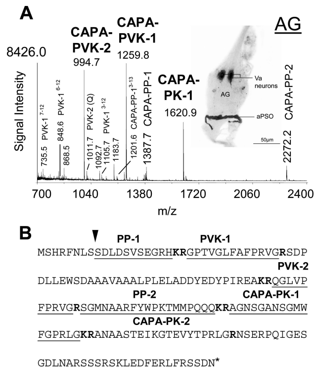
Figure 1. Detection of putative CAPA-peptides from Ae. aegypti by means of MALDI-TOF MS. (A) MALDI-TOF mass spectrum typical of an abdominal ganglion preparation with attached perisymphetic organ (aPSO). Only CAPA-peptides are labeled, and the most prominent mature products are given in bold. Note the complete absence of the ion signal of putative CAPA-PK-2 ([M + H]: 1920.0). The inset shows an abdominal ganglion immunostained with an anti-CAPA-PVK serum (Neupert, unpublished). (B) Sequence of the CAPA-precursor with the putative cleavage sites are labeled in bold. No signal peptide was predicted. Neuropeptides with mass match in (A) are underlined.
