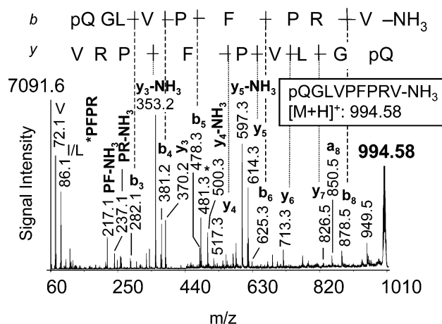
Figure 2. CID mass spectrum of the CAPA-peptide at [M + H]^+ : 994.58 Da. The fragments were analyzed manually and the resulting sequence is given in the inset. A number of fragment ions are labeled which confirmed the amino acid sequence of N-terminally blocked (pGlu) CAPA-PVK-2.
