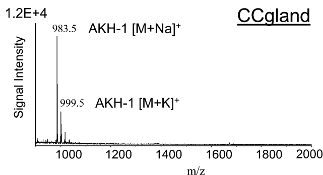
Figure 6. MALDI-TOF mass spectrum from the glandular portions of the corpora cardiaca. Only AKH-1 is detectable, ion signals of the putative AKH-2 are completely missing. AKH, adipokinetic hormone; CCgland, glandular portions of the corpora cardiaca.
