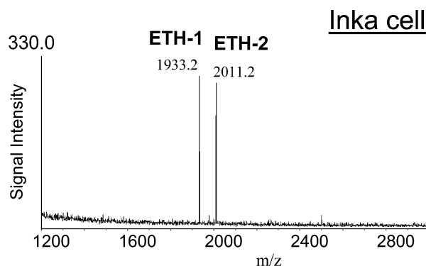
Figure 7. MALDI-TOF mass spectrum of a preparation of a lateral tracheal trunk (with Inka-cells) of an Ae. aegypti larvae. Two distinct ion signals representing the ETHs are marked. The synthesis and release of these (neuro)peptides is restricted to Inka-cells of larval stages.
