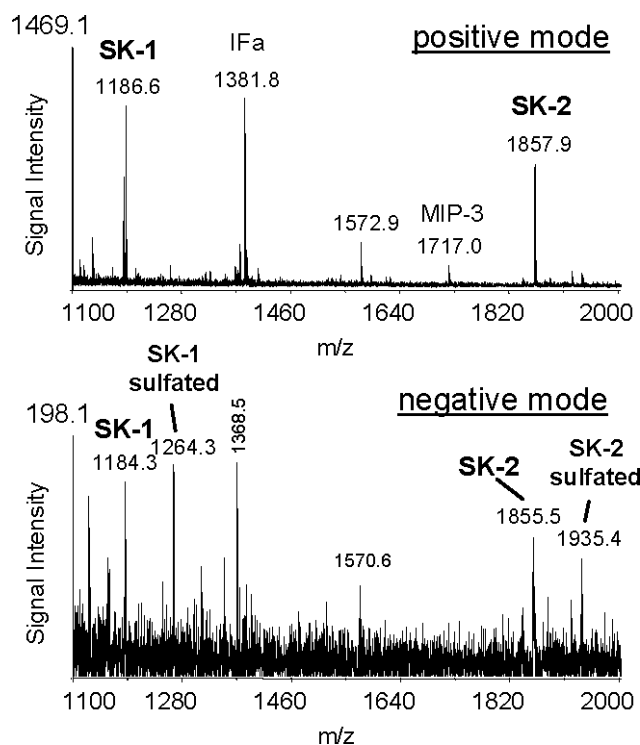
Figure 3. MALDI-TOF mass spectra of a preparation of brain tissue with fairly high concentrations of sulfakinins. The comparison of mass spectra in the positive and negative mode indicates the occurrence of the sulfate groups (mass difference of 80 Da). As already shown for other sulfakinins, 37 ions with sulfation are detectable in the negative mode only. The generally low amount of sulfakinins in the brain of Ae. aegypti limited the quality (signal-to-noise) of the mass spectra in the negative mode.
