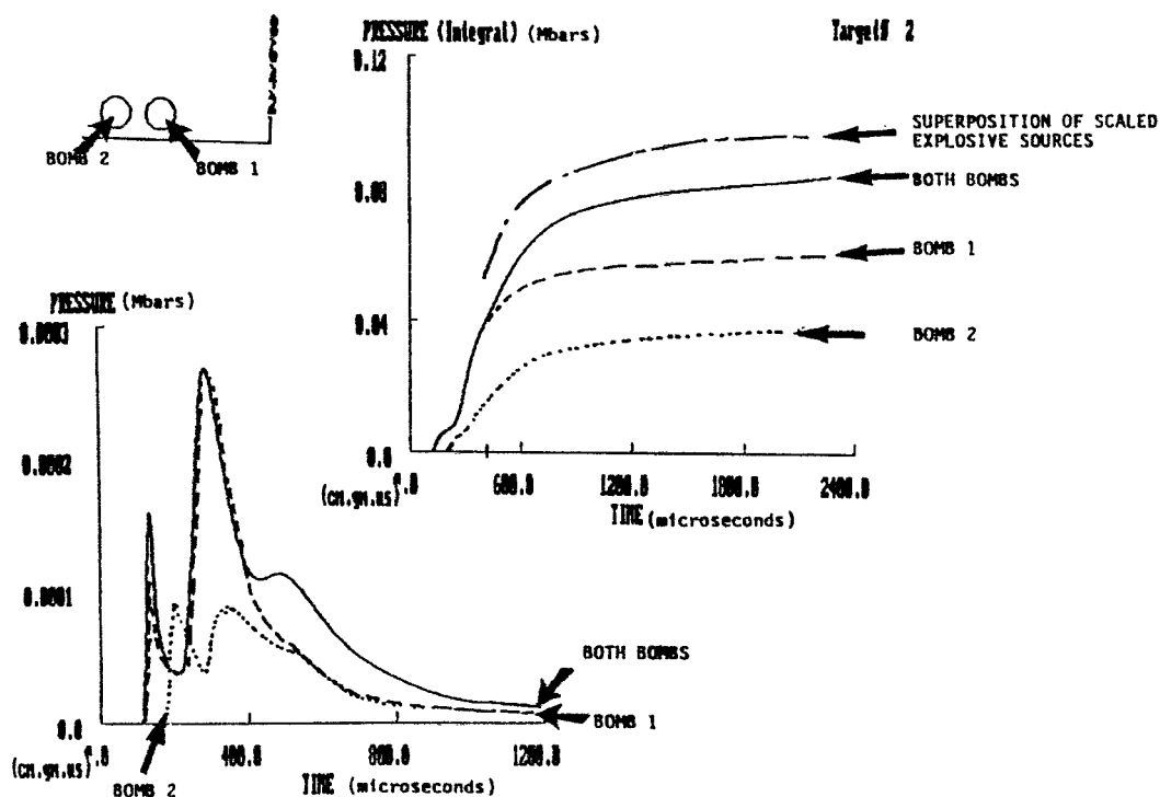
Figure 2. Pressure and Impulse Associated with Detonation of Two Mk82 Bombs Stacked Perpendicular to Ground Compared with Superposition of Single Bomb Detonations at Corresponding Locations
