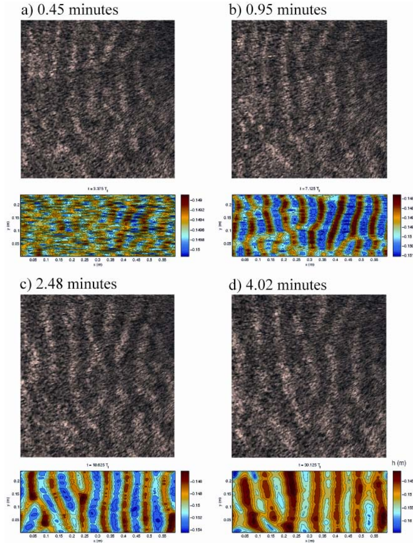
Figure 4: Comparison of bed elevations simulated with Chou and Fringer model (below) to sonar images(above) from experimental run 11 (wave velocity 39 cm/s and no current) at a) 0.45, b) 0.95, c) 2.48 and d) 4.02 minutes after run began. Run duration was 38 minutes.
