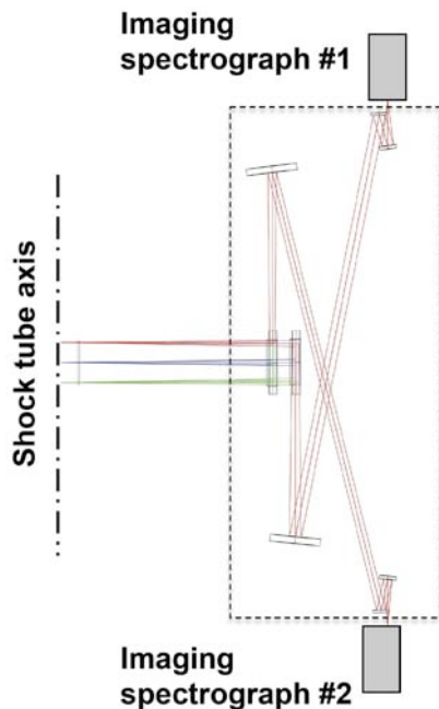
Figure 3: Optical configuration of spectrograph collection optics.
