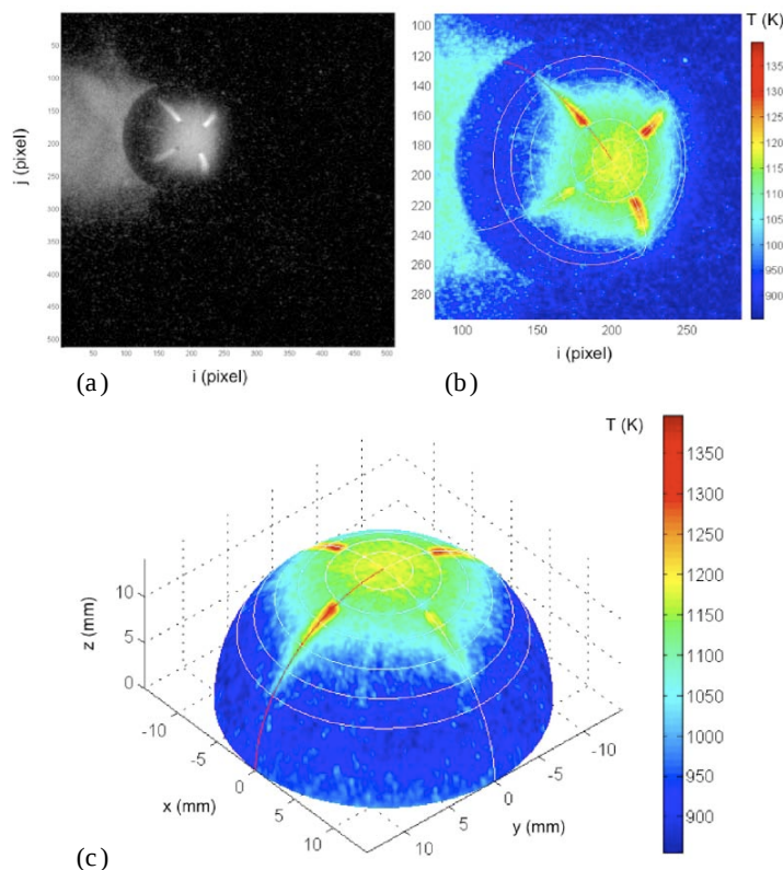
Figure 20: Hemispherical model with isolated roughness in flight through \text{CO}_2 at a pressure of 20.3 kPa and velocity 4.0 km/s. (a) ICCD image, (b) global surface temperature distribution with coordinate grid mapping, (c) temperature image after resection to 3D coordinate grid.
