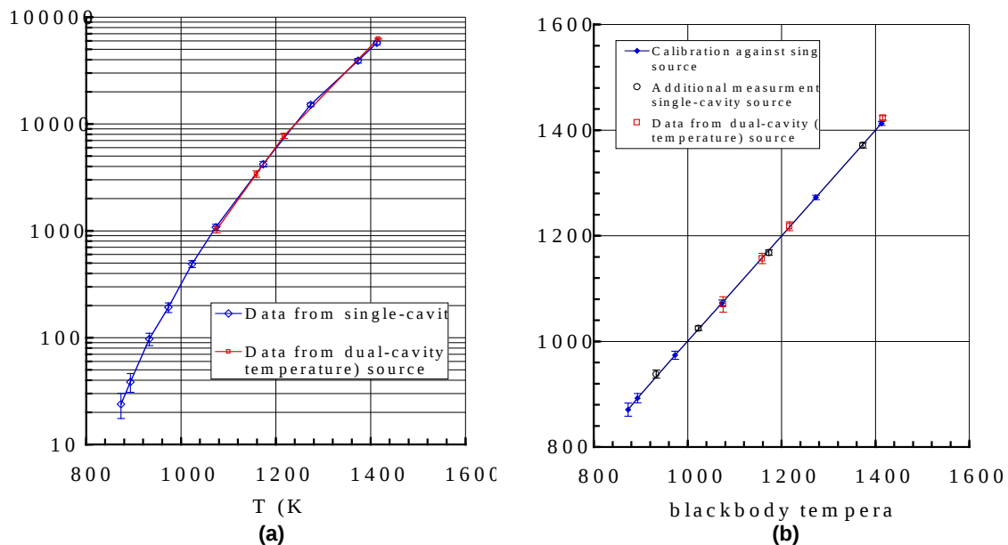
Figure 12: (a) Blackbody calibration data for an ICCD camera; (b) Response calibration applied to additional blackbody data.
