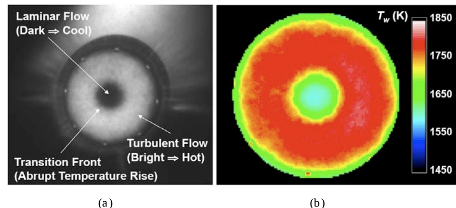
Figure 18: Pre-ablated graphite hemispherical model in flight in air at a pressure of 32.1 kPa and a velocity of 4.5 km/s. (a) ICCD camera image. (b) global surface temperature distribution.
