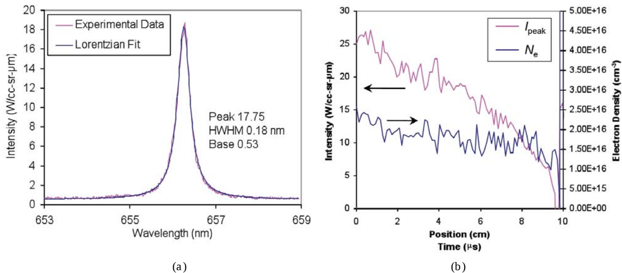
Figure 9: Stark broadening measurement of the H- \alpha line. (a) Spectral profile averaged over the equilibrium region and Lorentzian fit to the lineshape. The electron density of 1.8 \times 10^{16} \text{ cm}^{-3} was determined from the fitted width. (b) Spatiotemporal trend of peak radiance and electron density.
