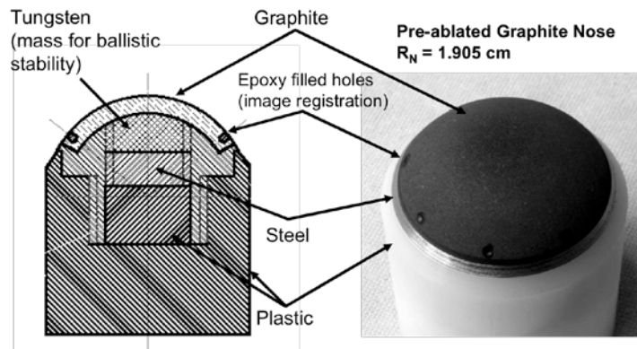
Figure 17: Engineering drawing and photograph of pre-ablated graphite hemispherical nosetip model.
