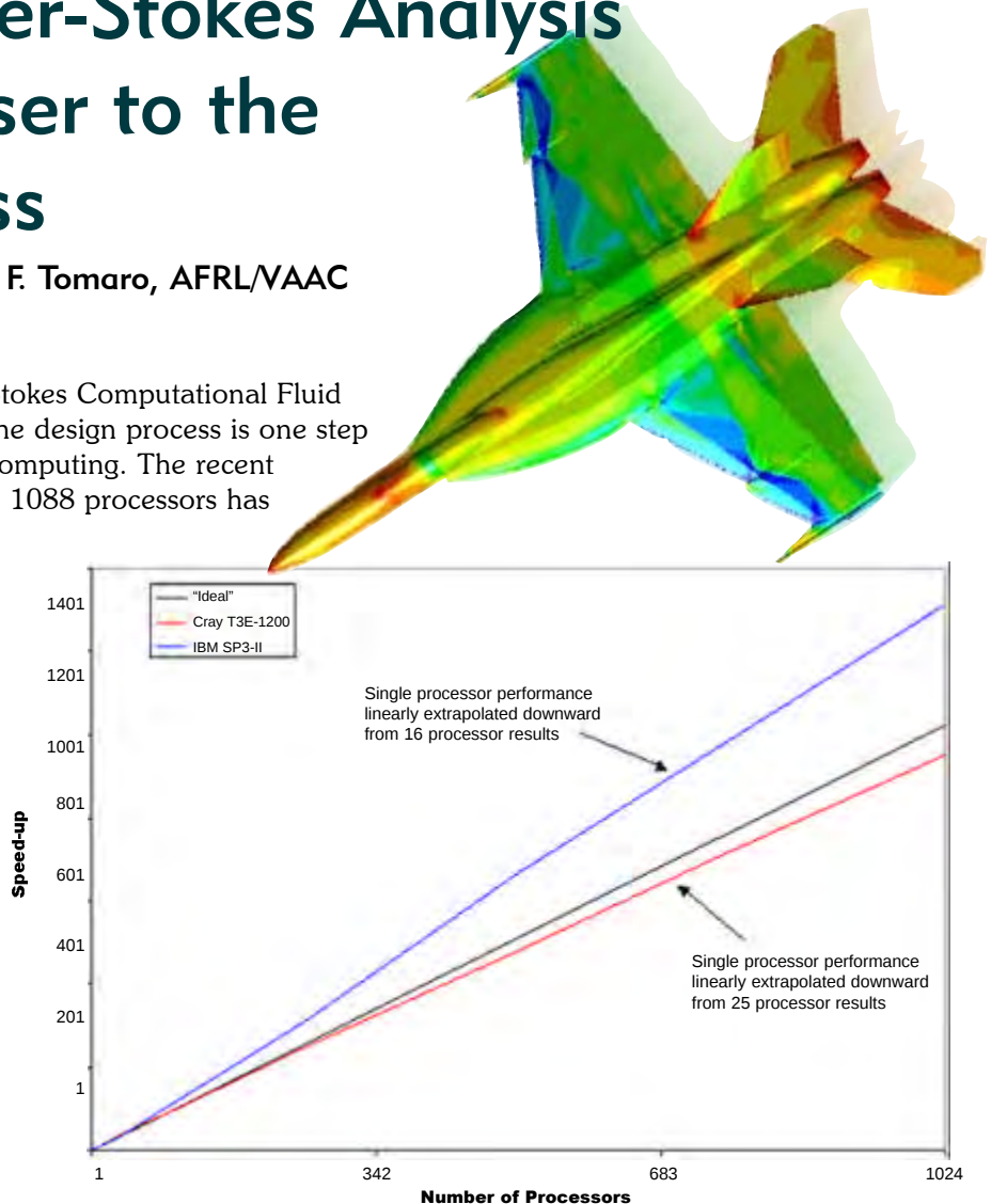
Figure 1. Speed-up for a large problem (3.17 million cells) for a benchmark run.
